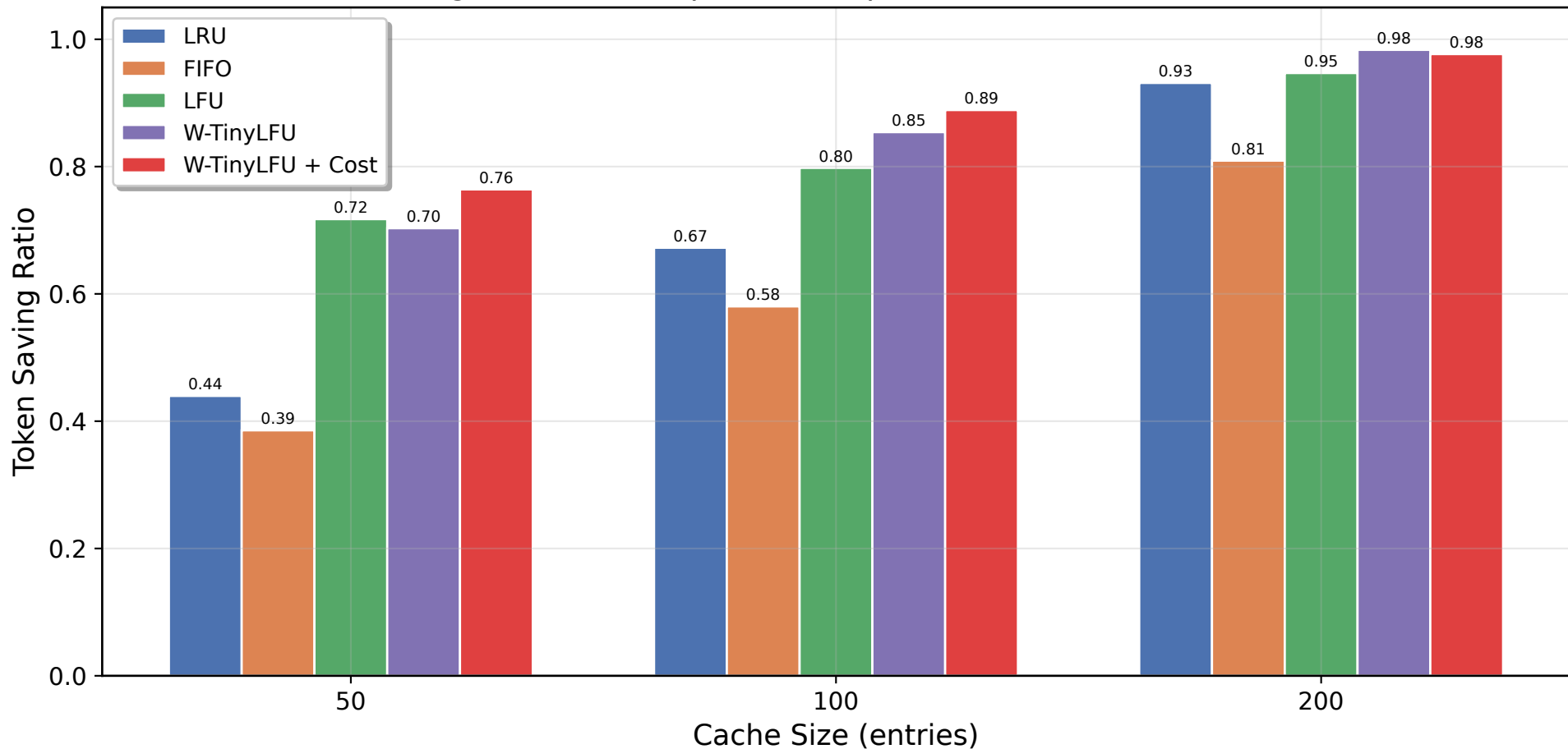
Token Saving Ratio by Eviction Policy (higher = more expensive responses retained in cache)
