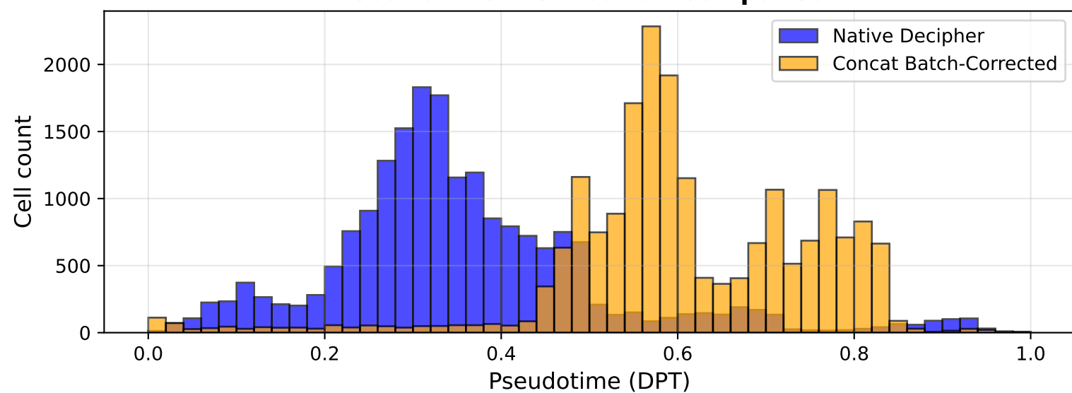
Pseudotime Distribution Comparison
