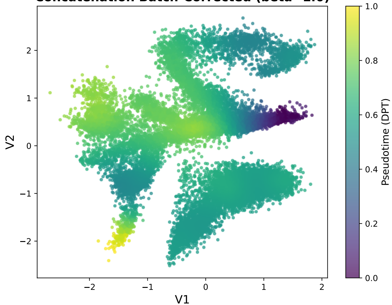
Concatenation Batch-Corrected (beta=1.0)
