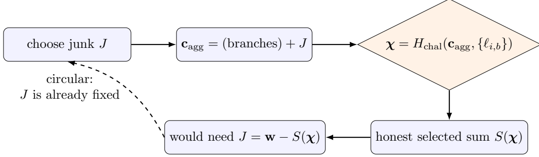
Figure 3: The fixpoint wall. Aiming the peeled sum at a target \mathbf{w} requires junk that cancels a challenge-dependent honest sum; the junk is committed before the challenge exists. Resolving the cycle is a search: guess the challenge pattern, set the junk accordingly, and hope the hash returns the guessed pattern.
