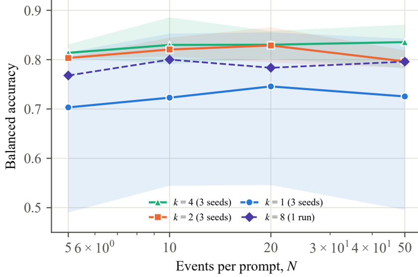
Figure 7: Balanced accuracy against the number of events for k = 1, 2 and 4 virtual tokens per event (lines: mean of three seeds; bands: seed range) and k = 8 (one run). The wide band at k = 1 is one failed run.
