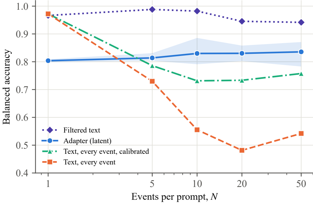
Figure 5: Balanced accuracy against the number of events per prompt on the class-balanced test windows. The shaded band is the range of the three adapter seeds. Filtered text is the most accurate arm; text with every event listed degrades as events are added and calibration recovers only part of the loss.
