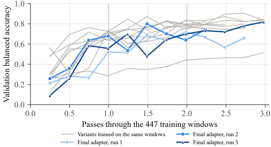
Figure 8: Validation balanced accuracy against passes through the 447 training windows, for the three runs of the final adapter and nine runs of variants trained on the same windows (exploratory; no test data). Most runs reach their best checkpoint within two passes and stop early; a few are still improving at the three-pass limit. The lowest grey curve is the one-token run that failed to learn the task.
