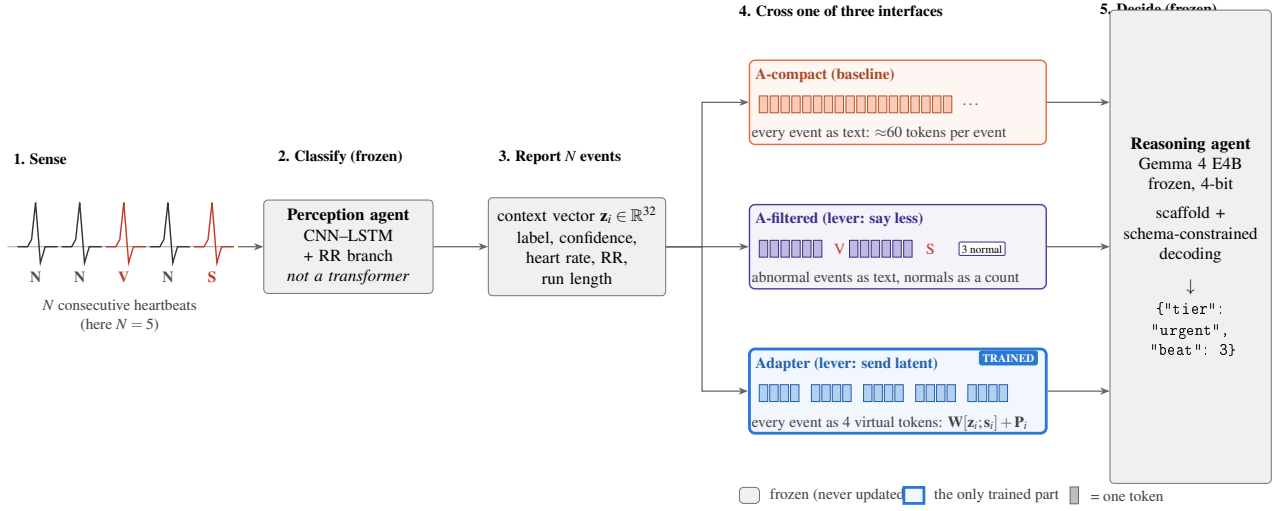
Figure 1: System overview. A perception agent that is not a transformer classifies each heartbeat, and the events of a window (abnormal beats in red) cross one of three interfaces to a frozen reasoning agent. Each small square is one token: text grows with every event (about 60 tokens each), the filter lists only abnormal events and counts the rest, and the adapter sends four virtual tokens per event. Grey boxes are frozen; only the adapter (blue) is trained. Sender, receiver and decoding are identical across arms, and the message sizes are the measured medians of Section 5.
