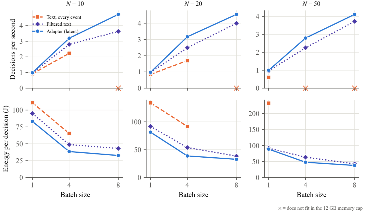
Figure 4: Throughput (top) and GPU energy per decision (bottom) when requests are batched, for 10, 20 and 50 events per prompt (final adapter, seed 101). A cross marks a configuration that did not fit in the memory cap of the 12 GB card. Filtered text at batch eight is plotted from the batches that fit, which are its shortest prompts.
