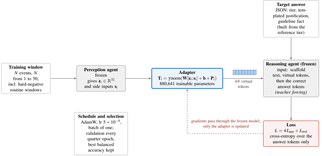
Figure 2: How the adapter is trained. The frozen perception agent supplies each event’s vector and side inputs, the adapter (blue, the only trained part) turns them into virtual tokens, and the frozen reasoning agent is run on the scaffold, the virtual tokens and the correct answer (teacher forcing). The loss weights the tier tokens four times as heavily as the rest. Gradients (dashed) flow back through the frozen model but update only the adapter.
