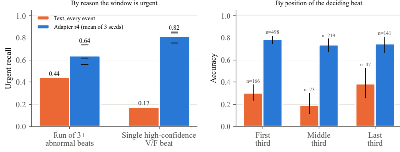
Figure 6: Urgent recall by the reason a window is urgent. Text with every event listed misses windows made urgent by a single high-confidence ventricular or fusion beat far more often than windows made urgent by a run; the adapter does not show this gap. Bars for the adapter are the mean of three seeds, with each seed’s value marked. Right: accuracy on non-routine windows with N \geq 10 by the position of the window’s most urgent beat; whiskers are 95% Wilson intervals, and the adapter counts are windows times three seeds. This panel is exploratory (not pre-registered) and is computed by scripts/position_effect.py .
