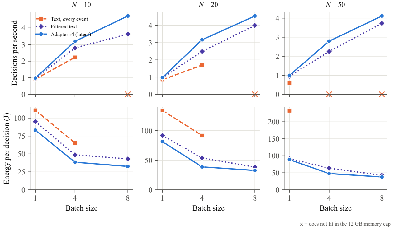
Figure 4: Throughput (top) and GPU energy per decision (bottom) when requests are batched, for 10, 20 and 50 events per prompt (adapter: recipe r4, seed 101). A cross marks a configuration that did not fit in the memory cap of the 12 GB card. Filtered text at batch eight is plotted from the batches that fit, which are its shortest prompts.
