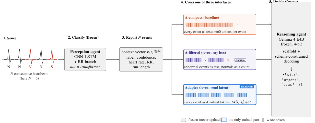
Figure 1: System overview. A perception agent that is not a transformer classifies each heartbeat, and the events of a window (abnormal beats in red) cross one of three interfaces to a frozen reasoning agent. Each small square is one token: text grows with every event (about 60 tokens each), the filter lists only abnormal events and counts the rest, and the adapter sends four virtual tokens per event. Grey boxes are frozen; only the adapter (blue) is trained. Sender, receiver and decoding are identical across arms, and the message sizes are the measured medians of Section 5.
