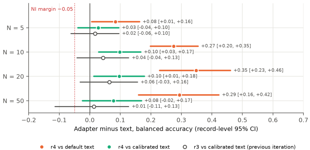
Figure 5. The comparisons of Table 6. Dotted red line: non-inferiority margin. Hollow markers show the previous recipe (r3) against calibrated text.
