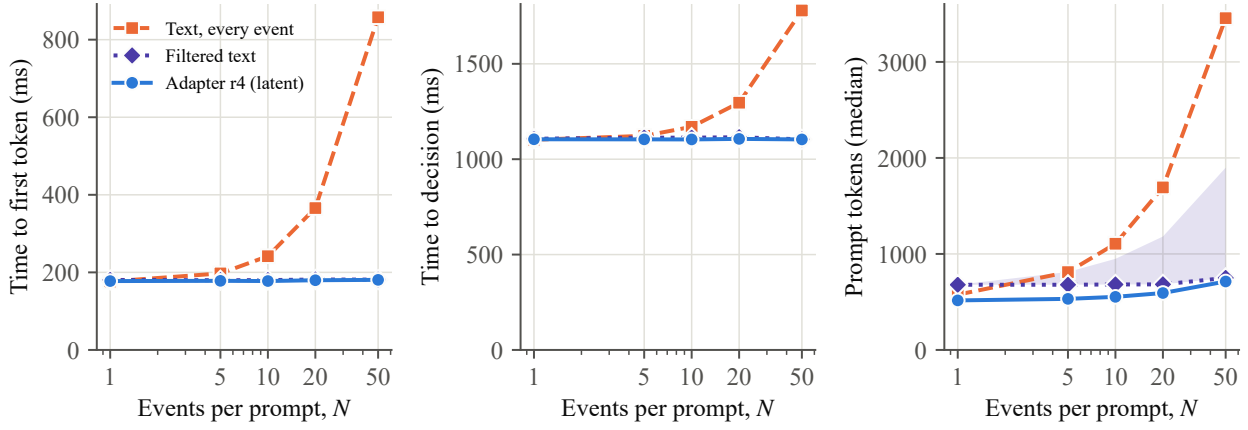
Figure 2: Cost of the three interfaces against the number of events per prompt (batch one, median of 21 windows per N ). The shaded band in the right panel is the 90th percentile of the filtered prompt: its length depends on content, whereas the adapter’s depends only on N . Time to decision is almost identical for filtered text and the adapter.
