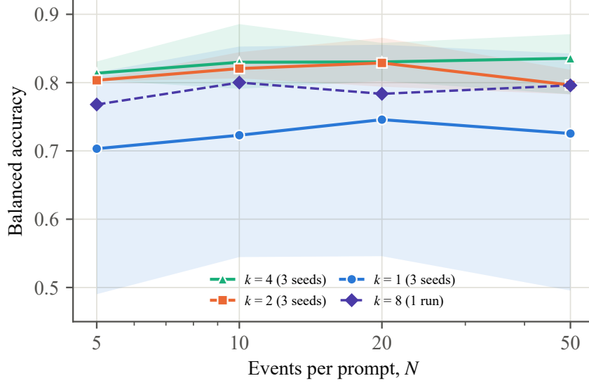
Figure 6: Balanced accuracy against the number of events for k = 1, 2 and 4 virtual tokens per event (lines: mean of three seeds; bands: seed range) and k = 8 (one run). The wide band at k = 1 is one failed run.
