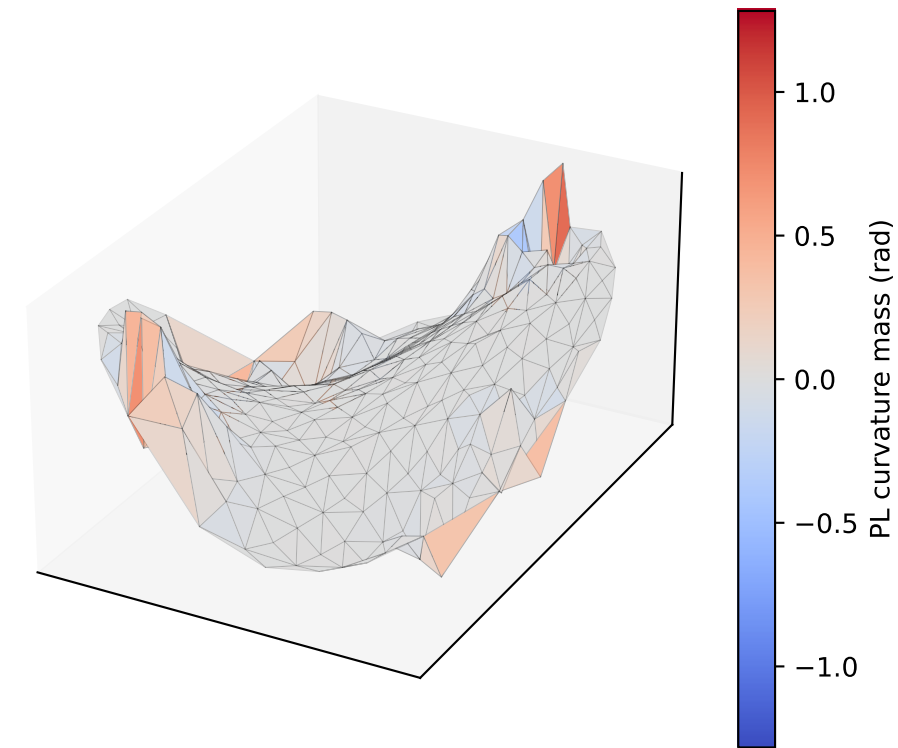
SAME SMOOTH R3 OUTPUT color = angle-defect PL curvature mass (rad; boundary omitted)
