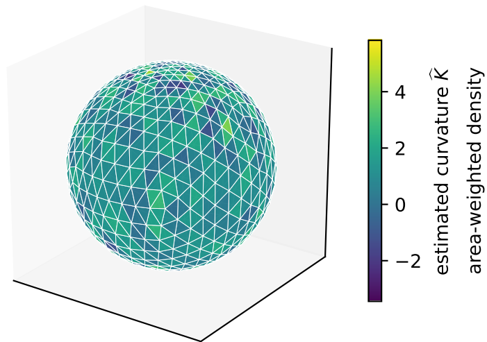
(a) Raw angle-deficit Gaussian curvature
