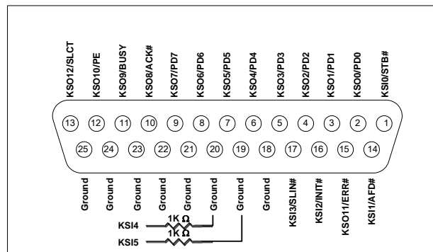
Figure 7-50. Parallel Port Female 25-Pin Connector
