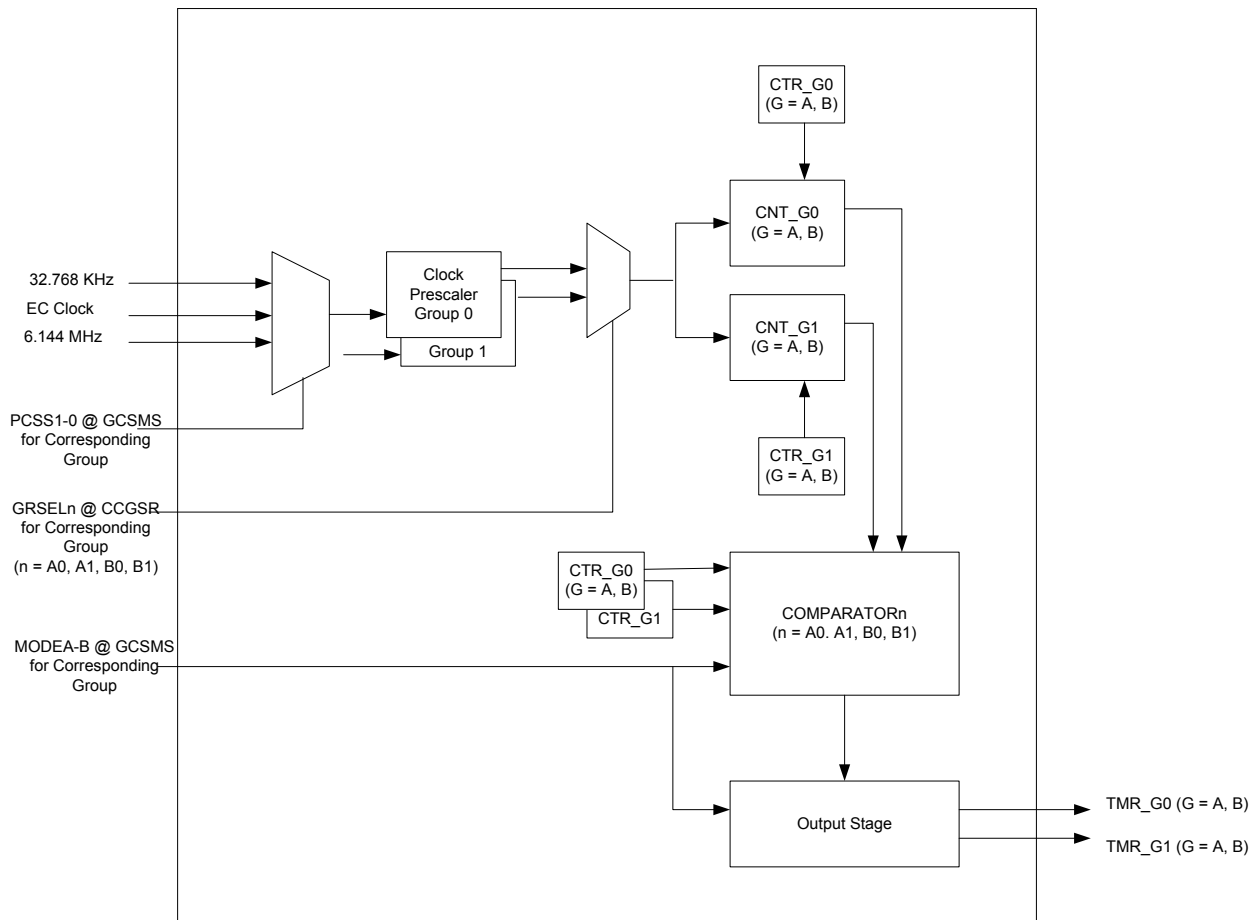
Figure 7-32. TMR Block Diagram
