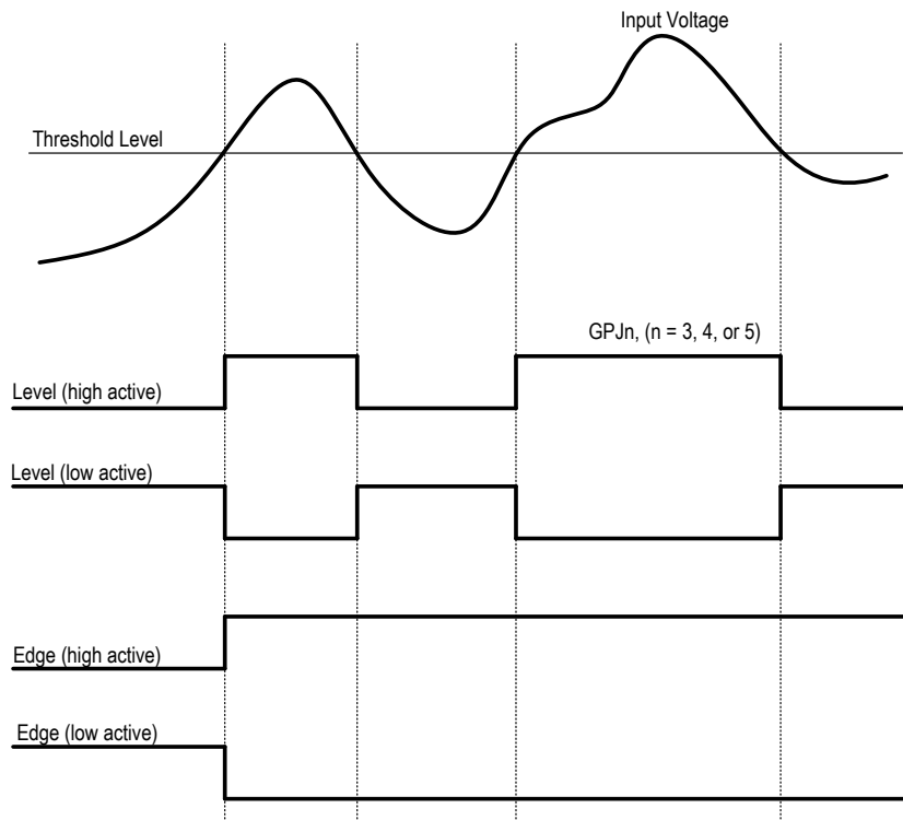
Figure 7-26. Voltage Comparator Operation Time
