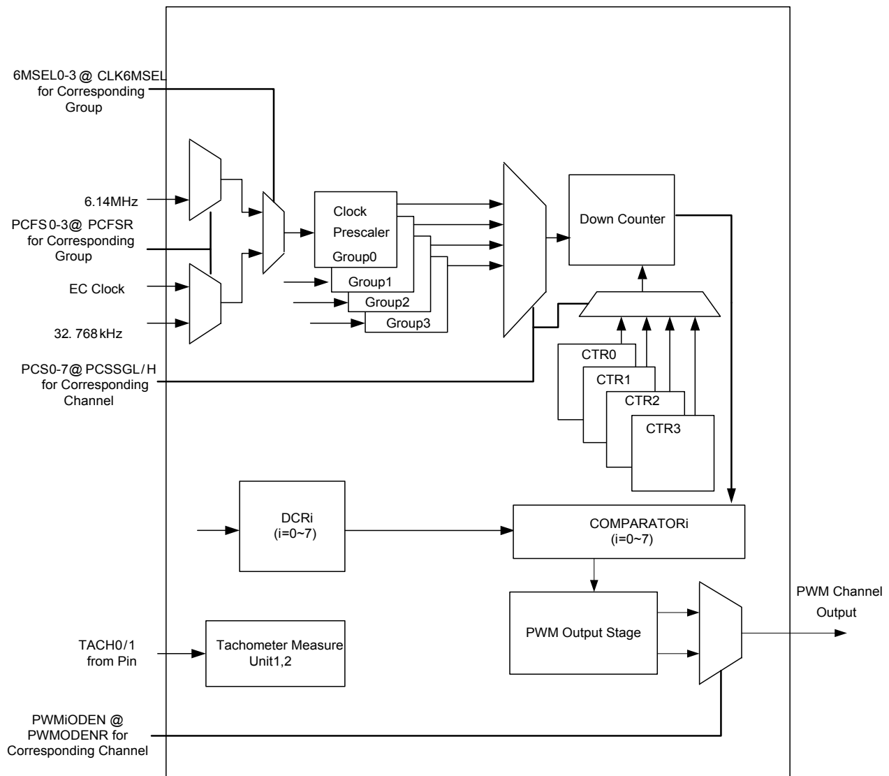
Figure 7-27. PWM Diagram
