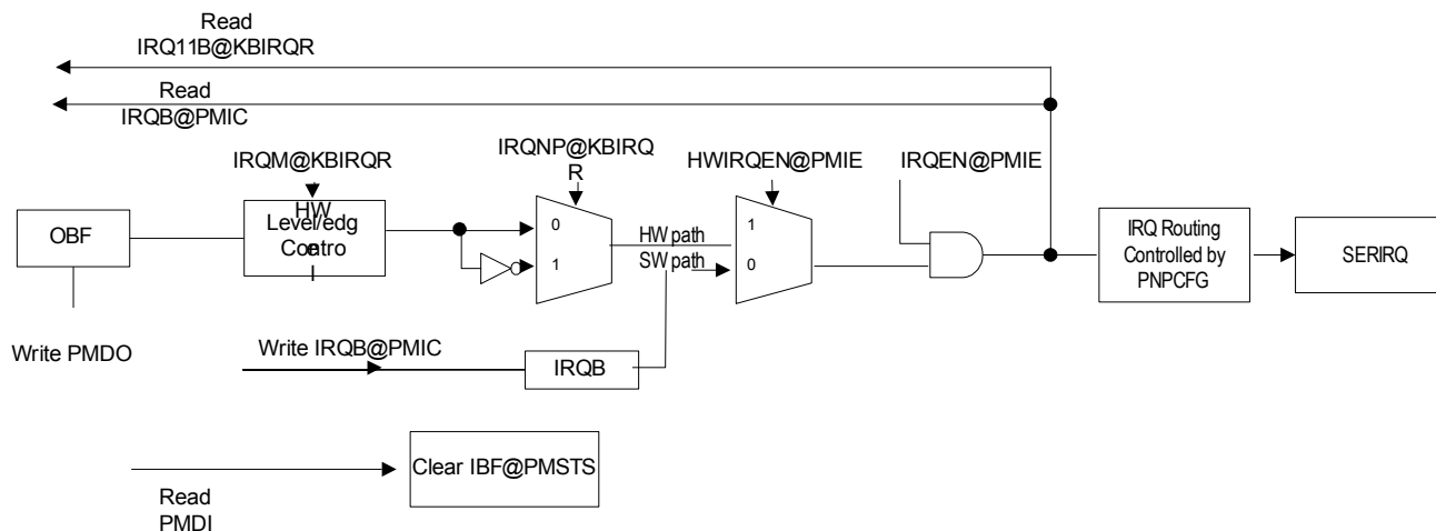
Figure 6-21. IRQ Control in PM Channel 3/4/5
