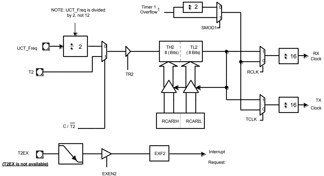
Figure 7-13. Timer 2 in Baud Rate Generator Mode
