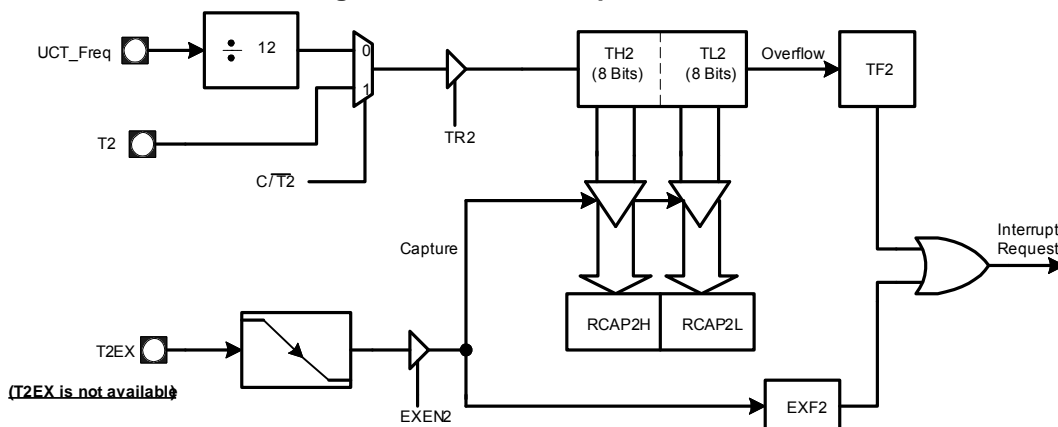
Figure 7-6. Timer 2: Capture Mode
