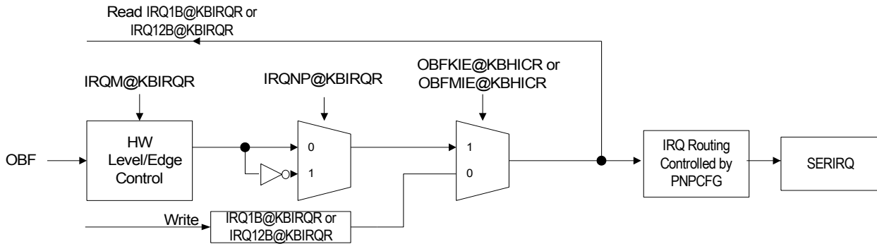
Figure 6-15. IRQ Control in KBC Module
