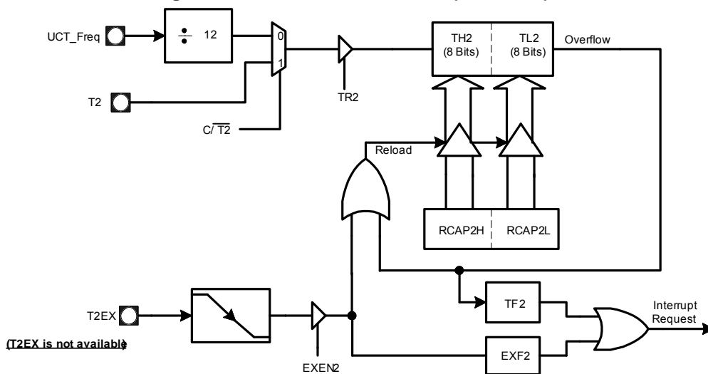
Figure 7-7. Timer 2: Auto Reload (DCEN = 0)
