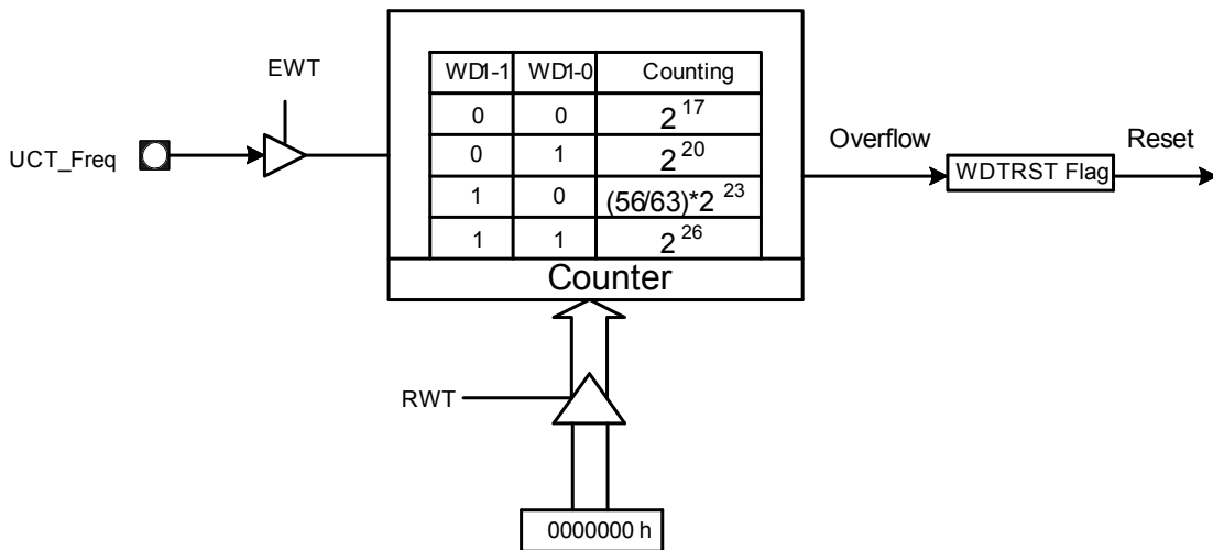
Figure 7-10. Watchdog Timer
