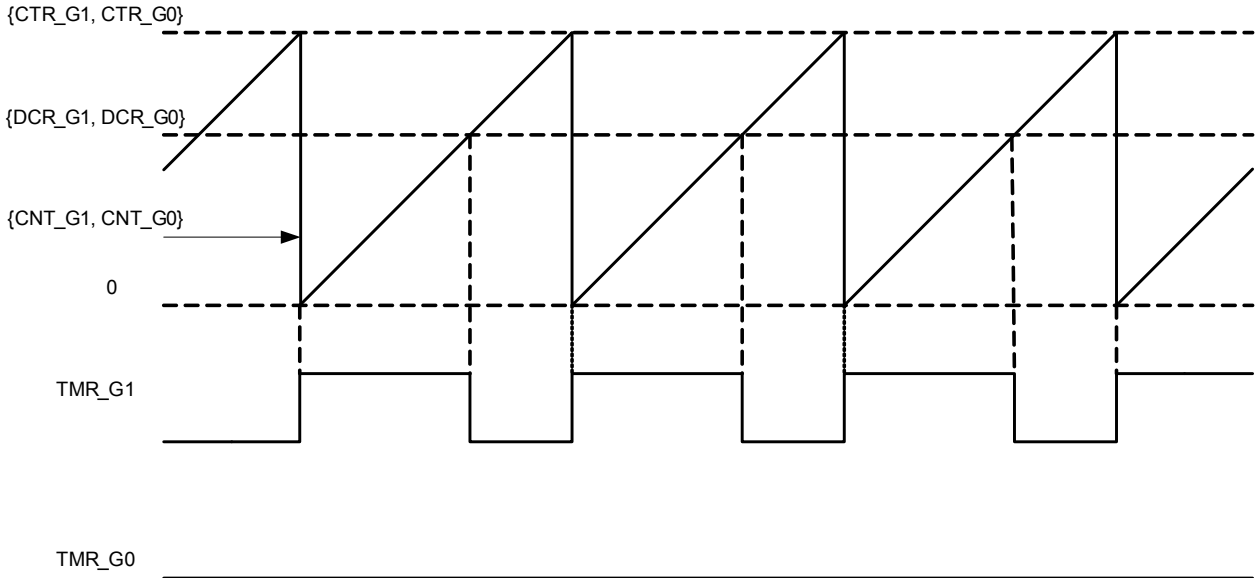
Figure 7-34. 16-bit Mode Waveform of Group G
