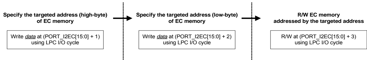
Figure 7-49. I2EC through Dedicated I/O Port Operation Flow
