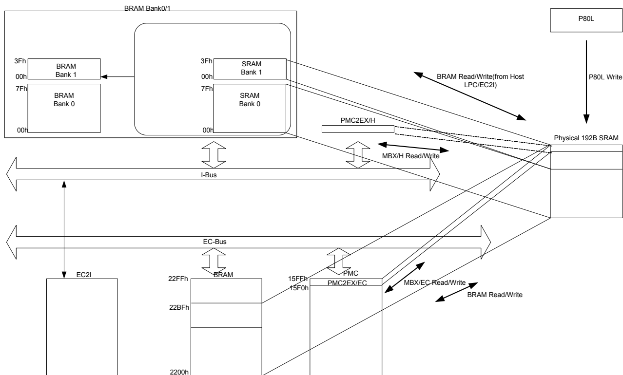
Figure 7-40. BRAM Mapping Diagram
