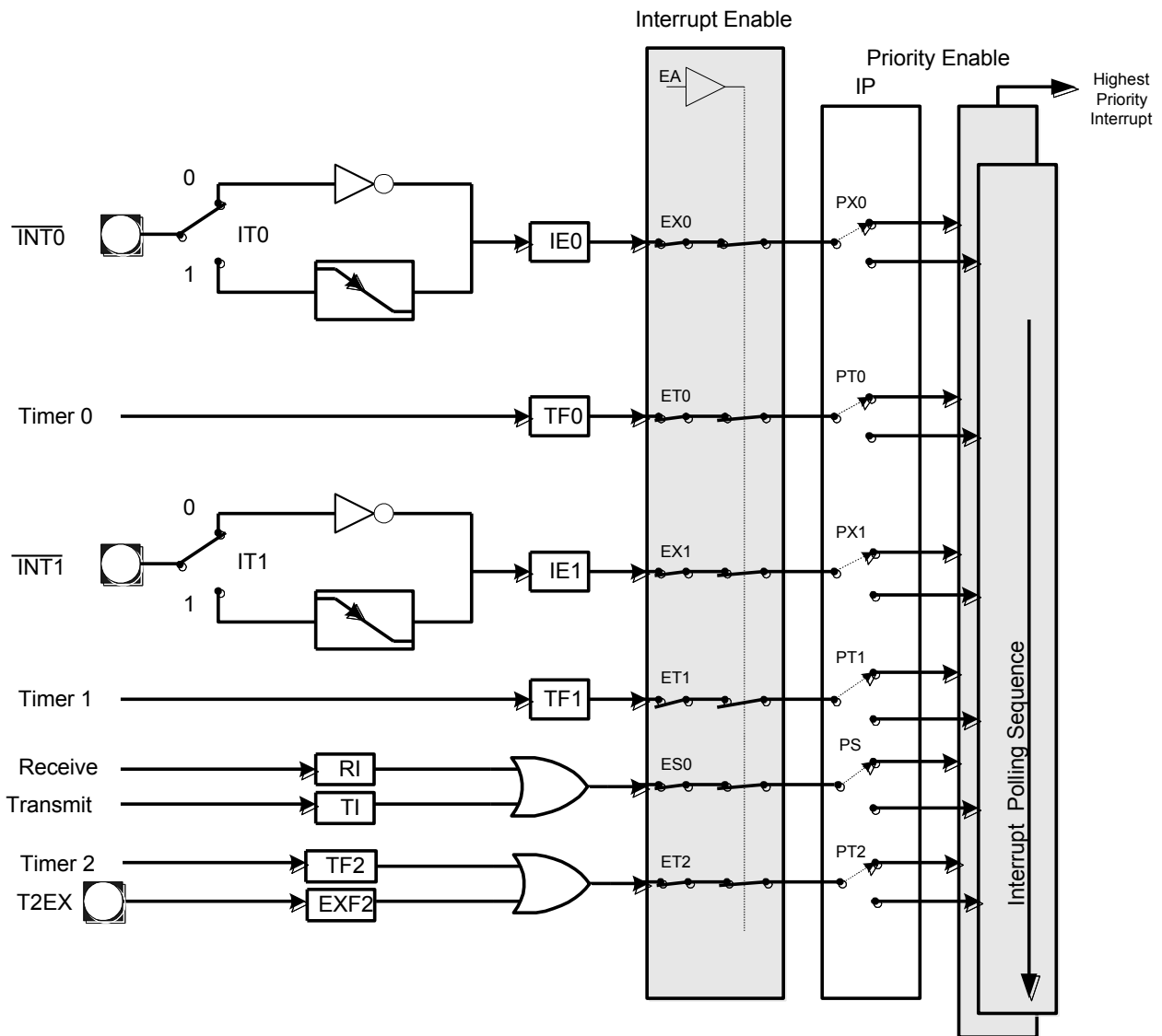
Figure 7-1. Interrupt Control System Configuration
