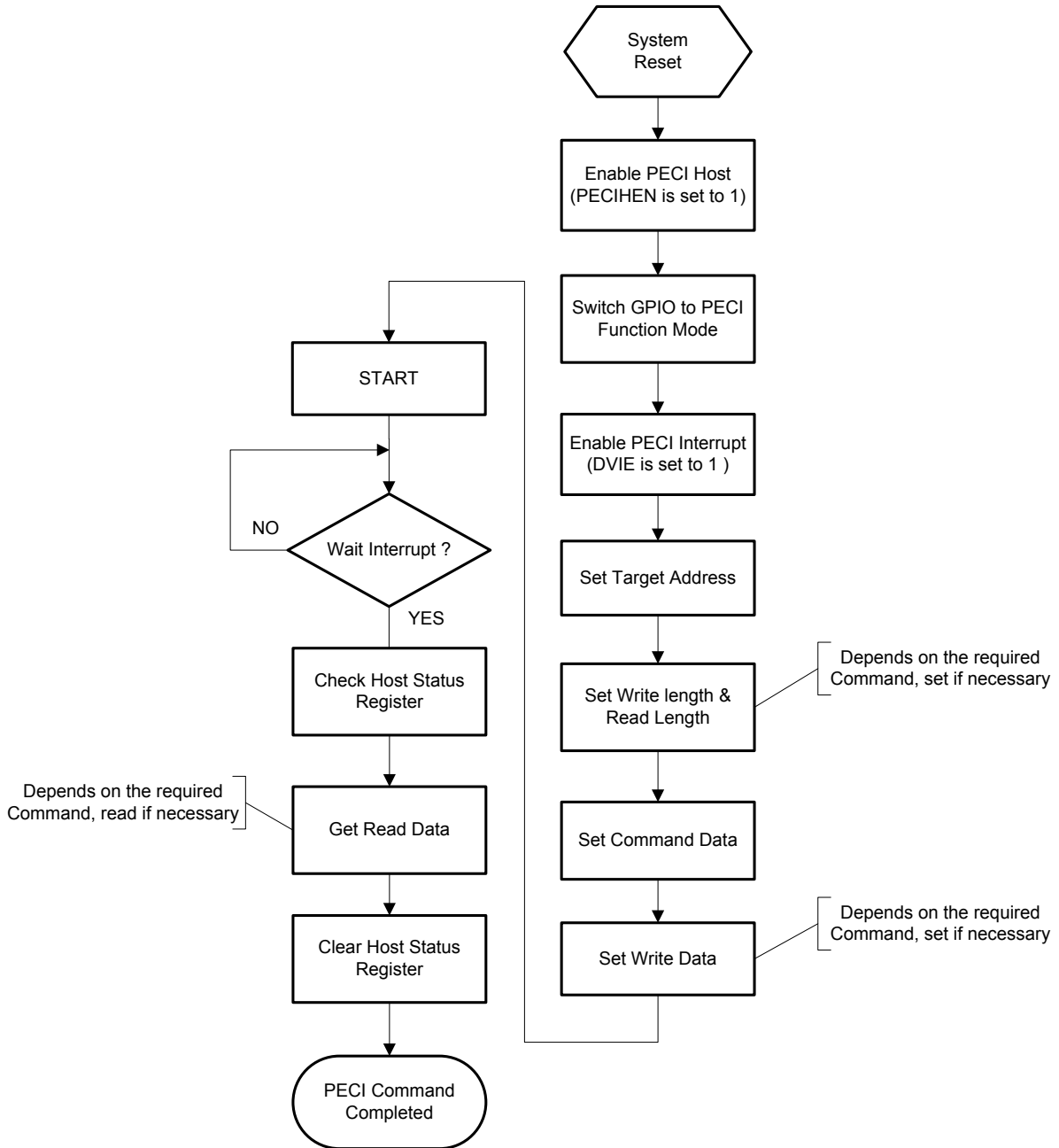
Figure 7-24. Program Flow Chart for Interrupt Mode
