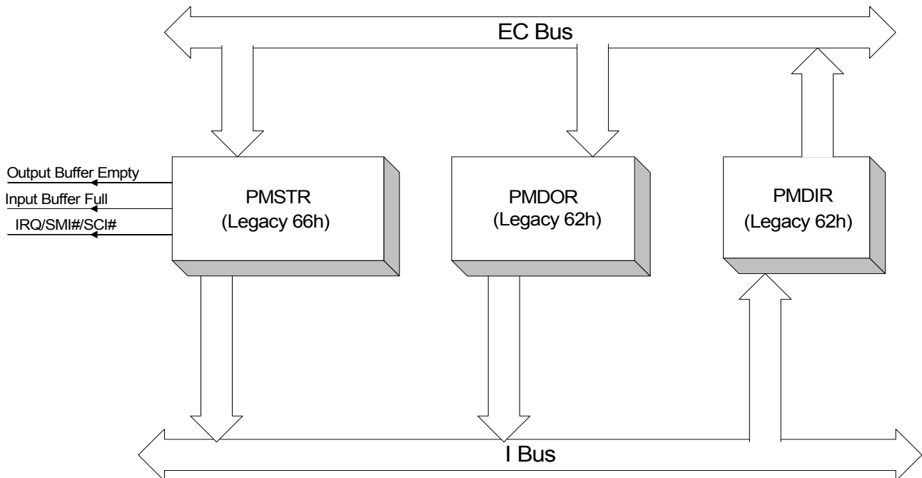
Figure 6-16. PMC Host Interface Block Diagram
