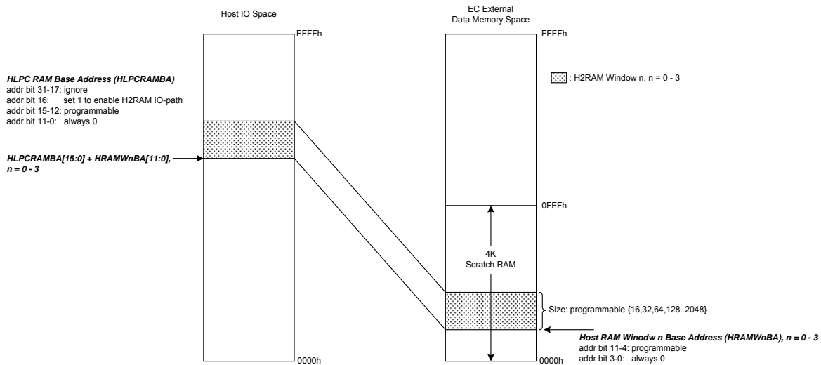
Figure 6-7. H2RAM-HLPC Mapping through LPC IO Cycles
