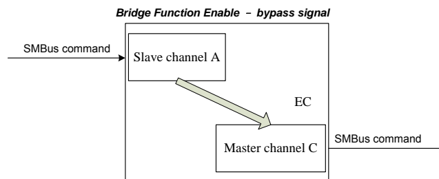
Figure 7-19. Diagram of SMBus Bridge Bypass Function
