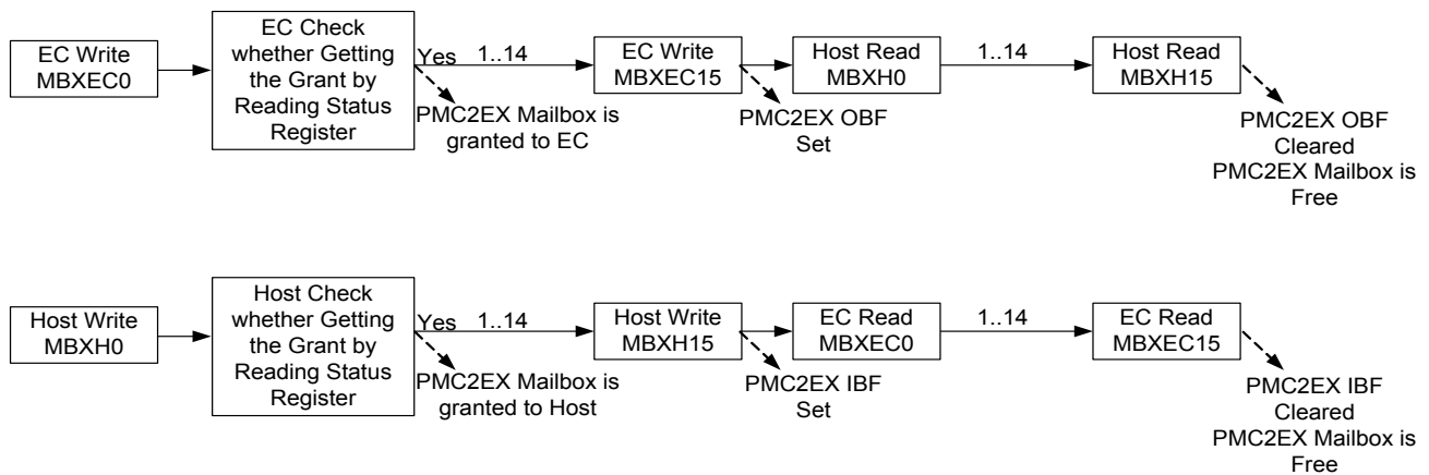
Figure 6-20. Typical PMC2EX Mailbox Operation
