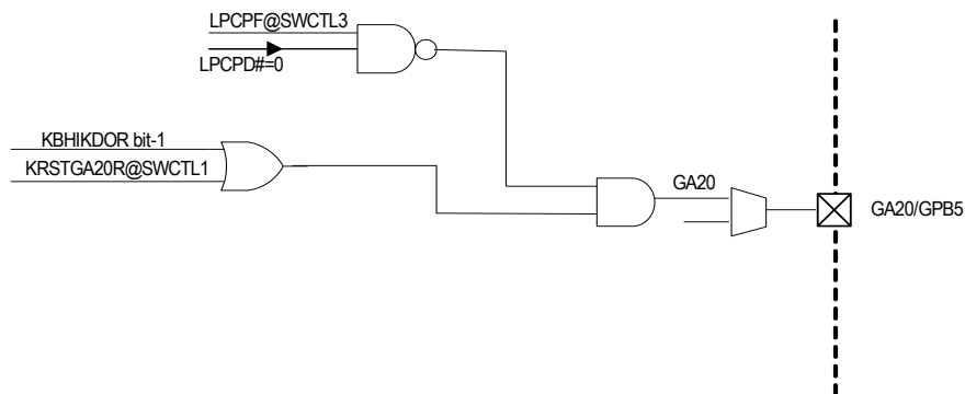
Figure 6-13. GA20 Output Scheme
