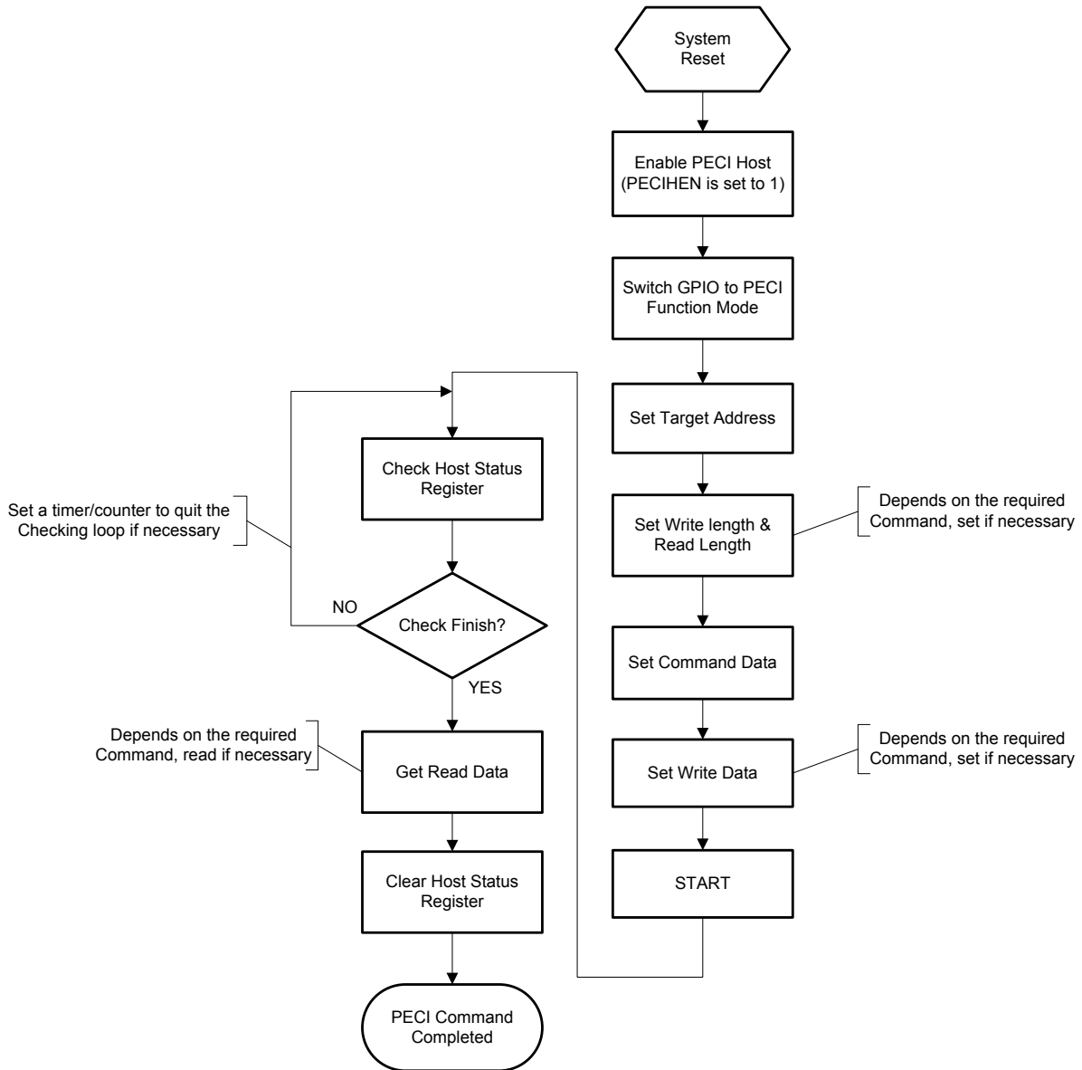
Figure 7-23. Program Flow Chart for Polling Mode
