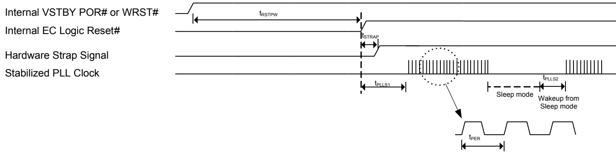
Figure 10-2. Reset Timing
