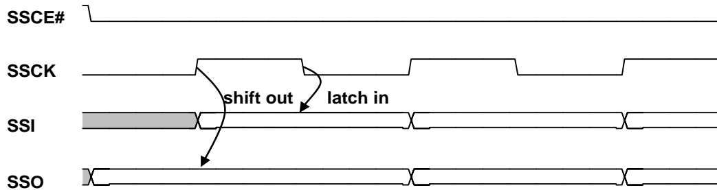
Figure 7-43. SPI Mode 1 Waveform
