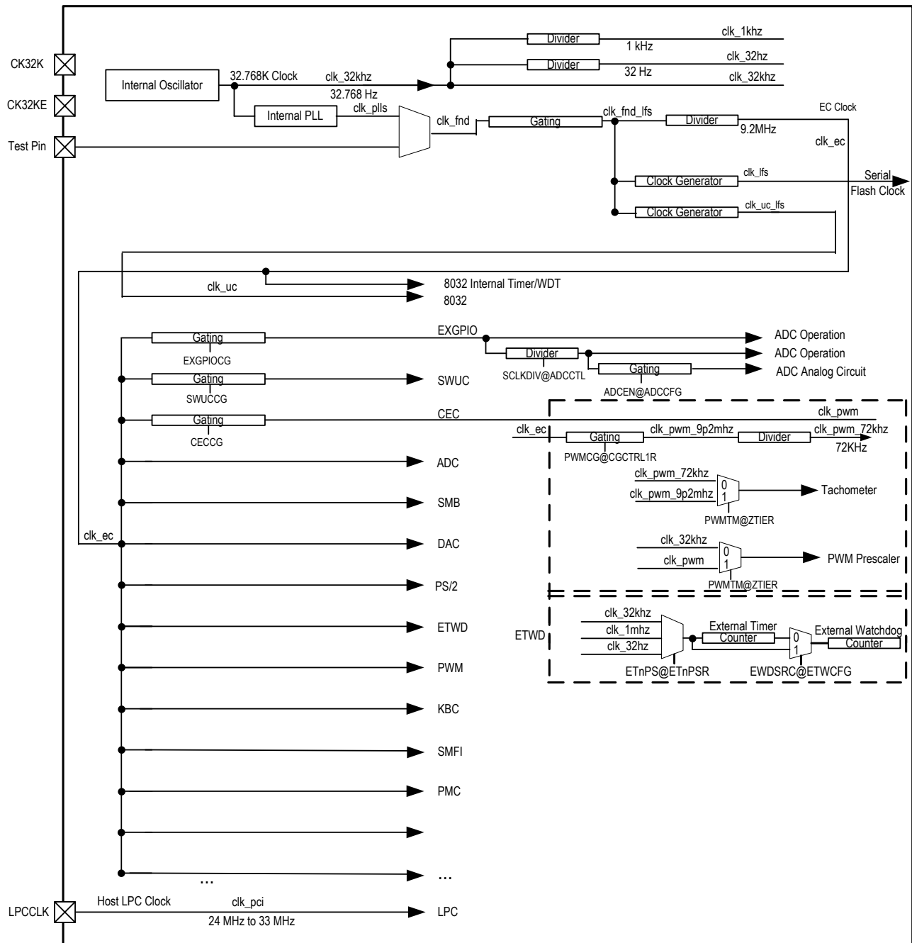
Figure 5-2. Clock Tree
