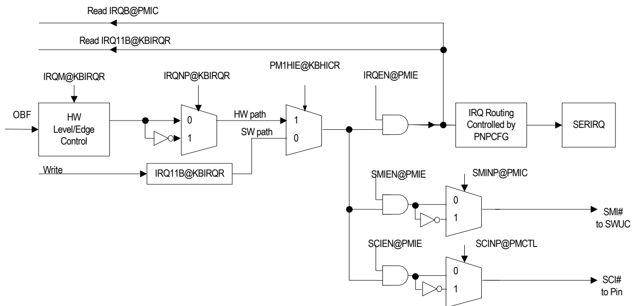
Figure 6-18. IRQ/SCI#/SMI# Control in PMC Compatible Mode
