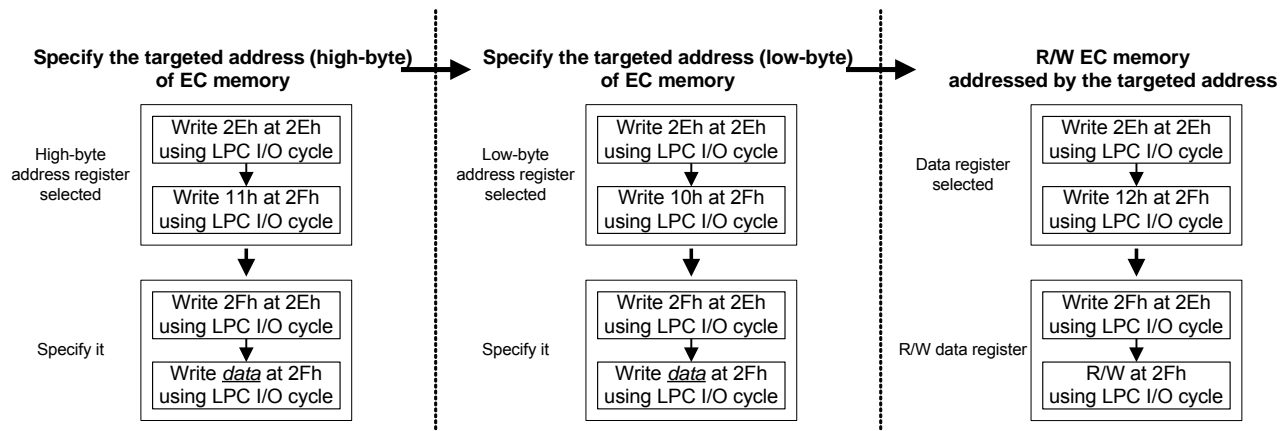
Figure 7-48. I2EC through 2Eh/2Fh I/O Port Operation Flow
