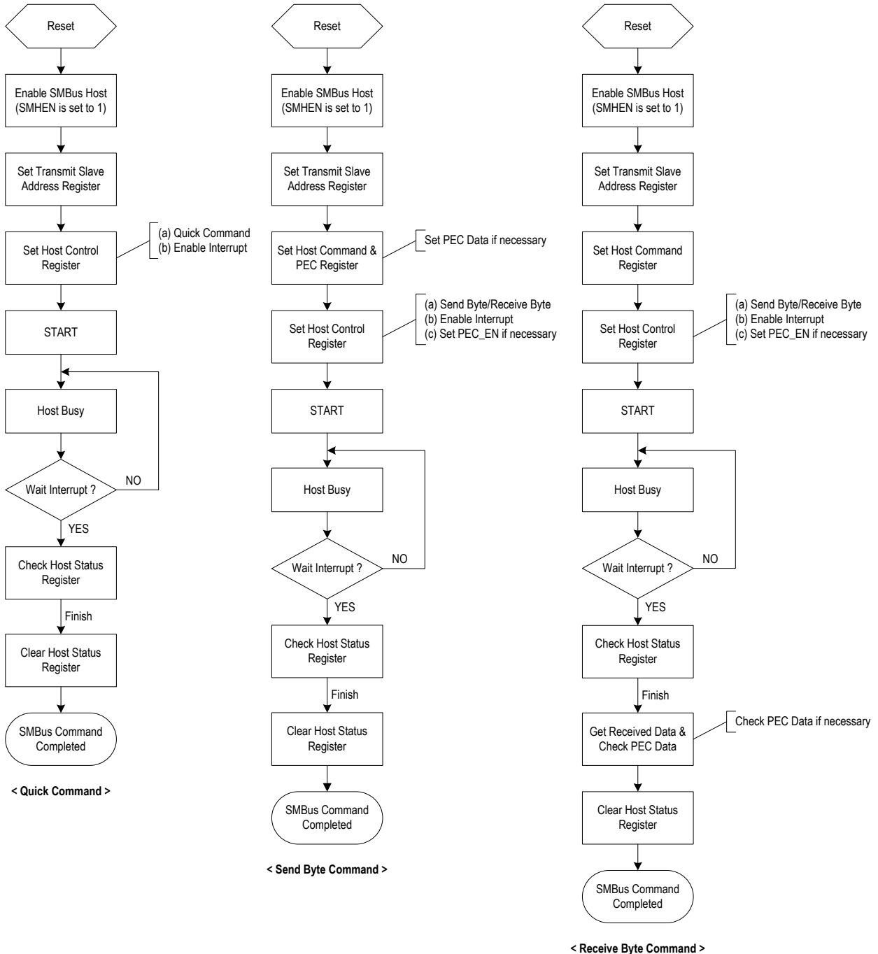
Figure 7-20. Program Flow Chart of SMBus Master Interface
