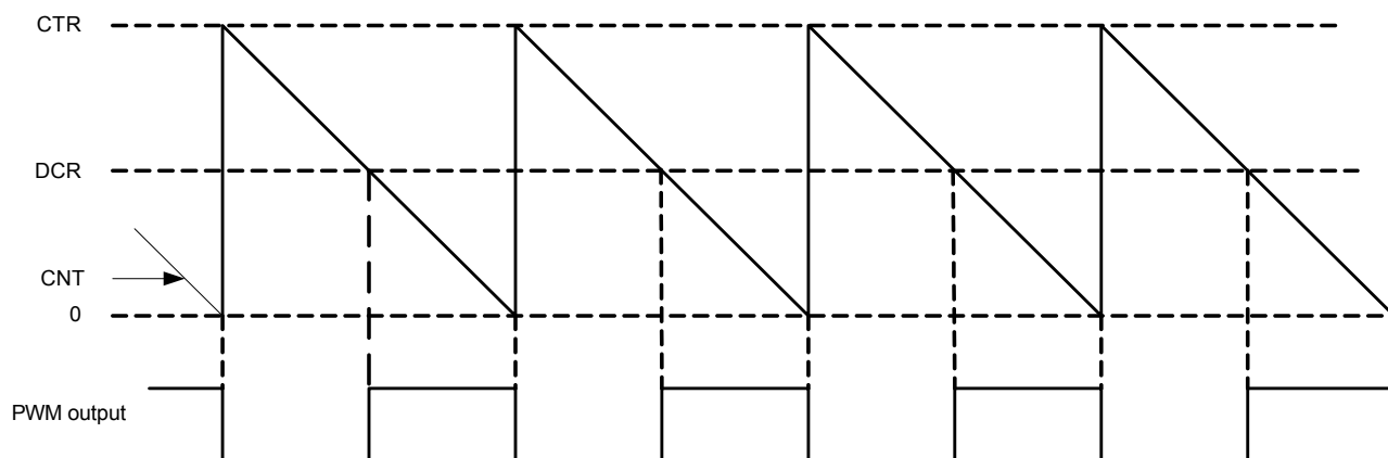
Figure 7-29. PWM Output Waveform
