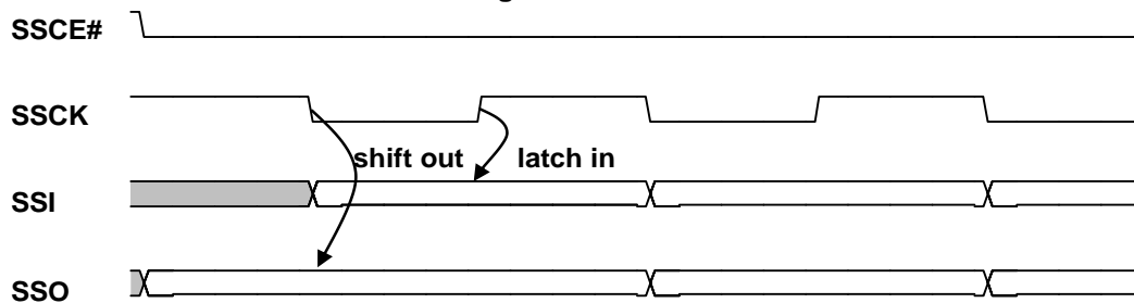
Figure 7-45. SPI Mode 3 Waveform
