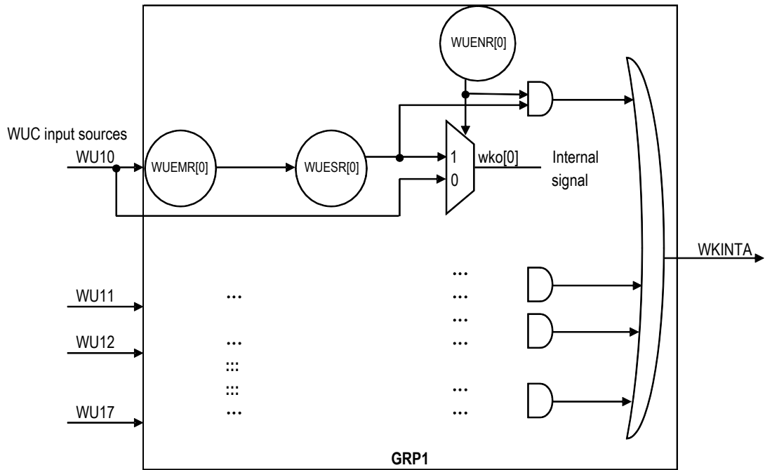
Figure 7-16. WUC Simplified Diagram
