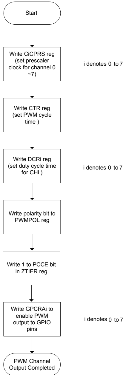
Figure 7-31. Program Flow Chart for PWM Channel Output
