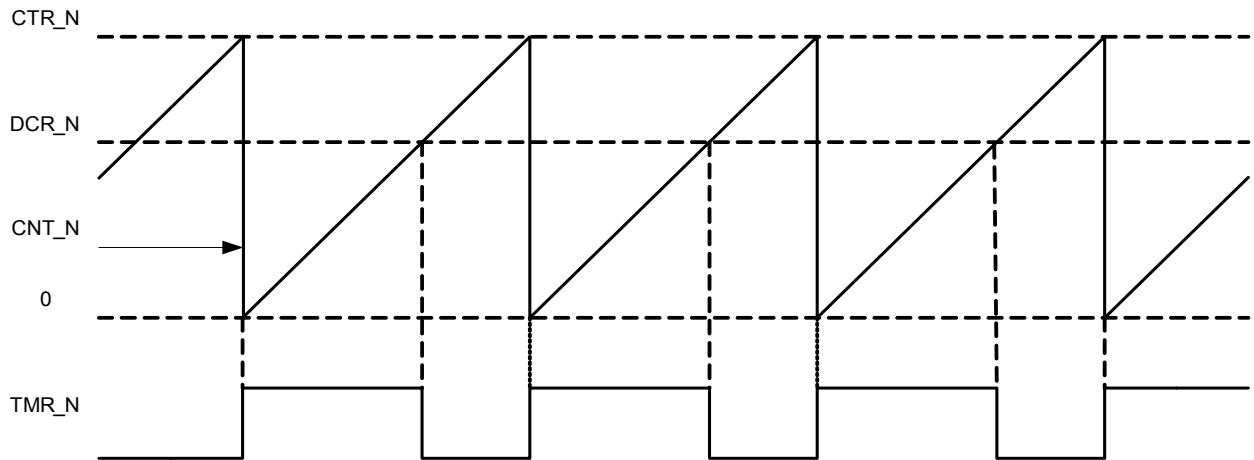
Figure 7-33. 8-bit Mode Waveform of Channel N
