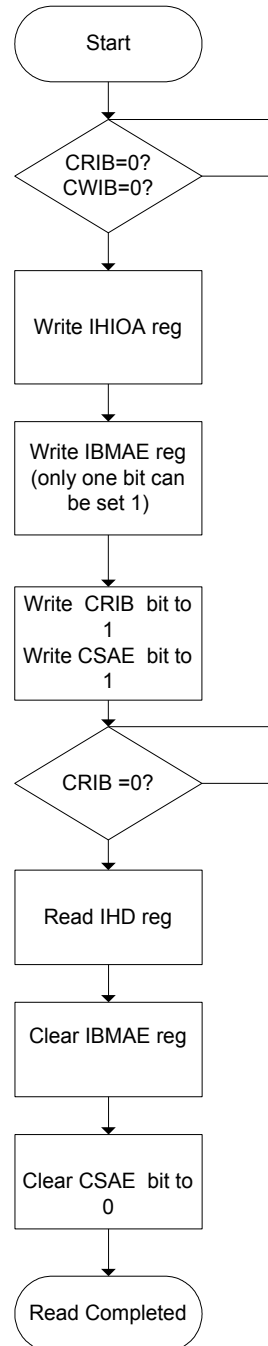
Figure 7-37. Program Flow Chart for EC2I Read
