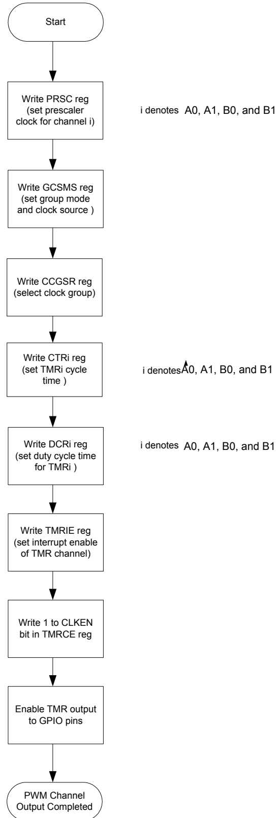
Figure 7-36. Program Flow Chart for TMR Channel Output
