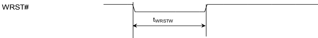
Figure 10-3. Warm Reset Timing
