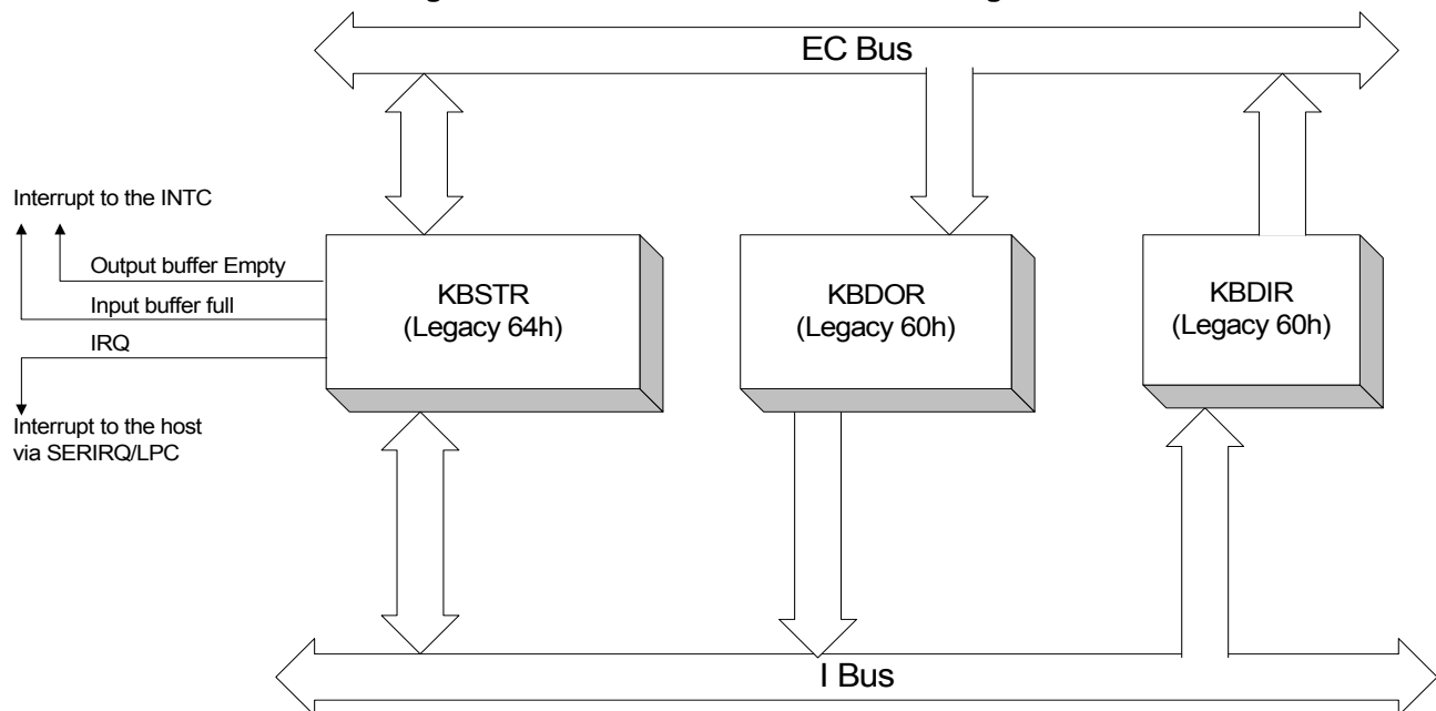
Figure 6-14. KBC Host Interface Block Diagram
