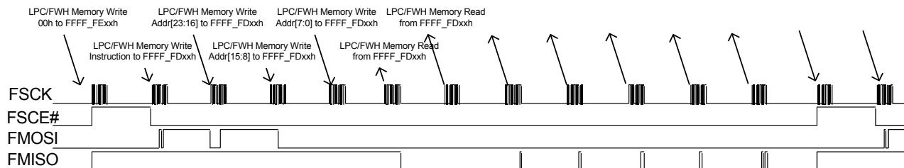
Figure 6-5. HLPC Follow Mode for Serial Flash (e.g. Fast Read Instruction)
