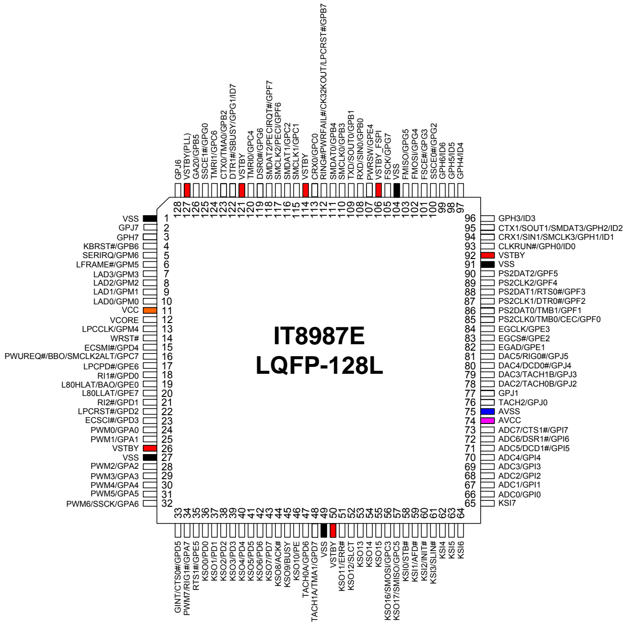
IT8987E Top View
