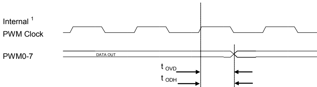
Figure 10-9. PWM Output Timing
