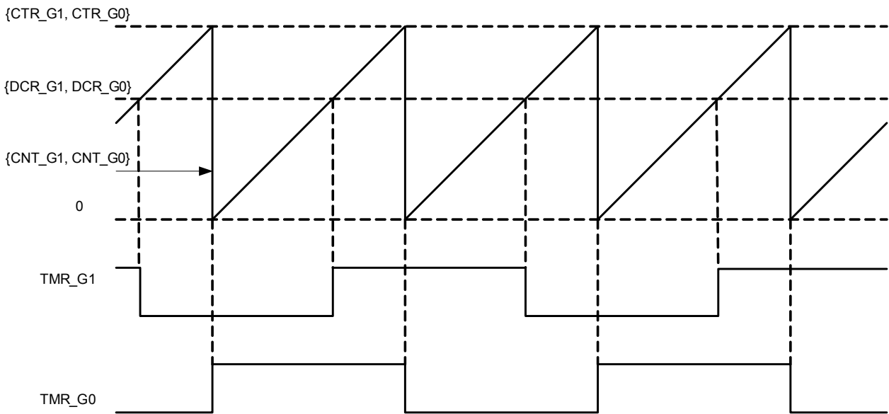
Figure 7-35. 16-bit Mode Waveform of Group N
