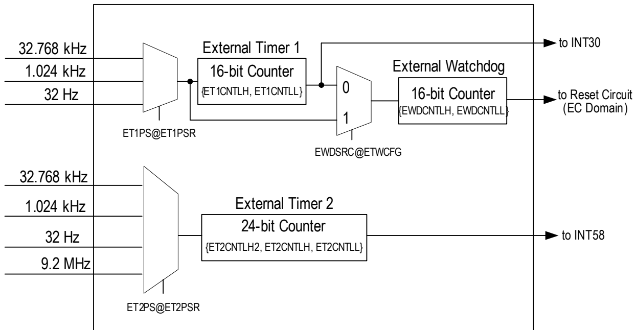
Figure 7-39. Simplified Diagram
