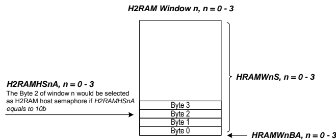
Figure 6-2. Location of H2RAM Host Semaphore
