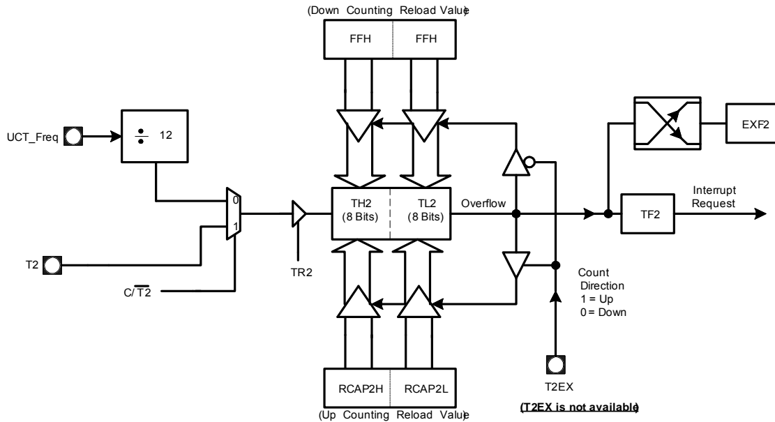
Figure 7-8. Timer 2: Auto Reload Mode (DCEN = 1)
