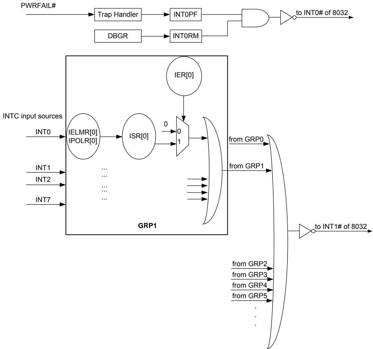
Figure 7-14. INTC Simplified Diagram
