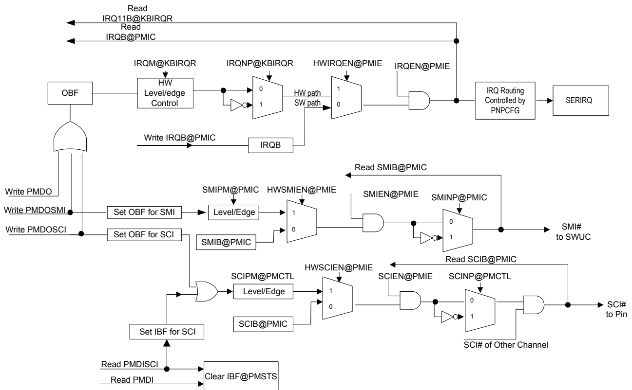
Figure 6-19. IRQ/SCI#/SMI# Control in PMC Enhanced Mode
