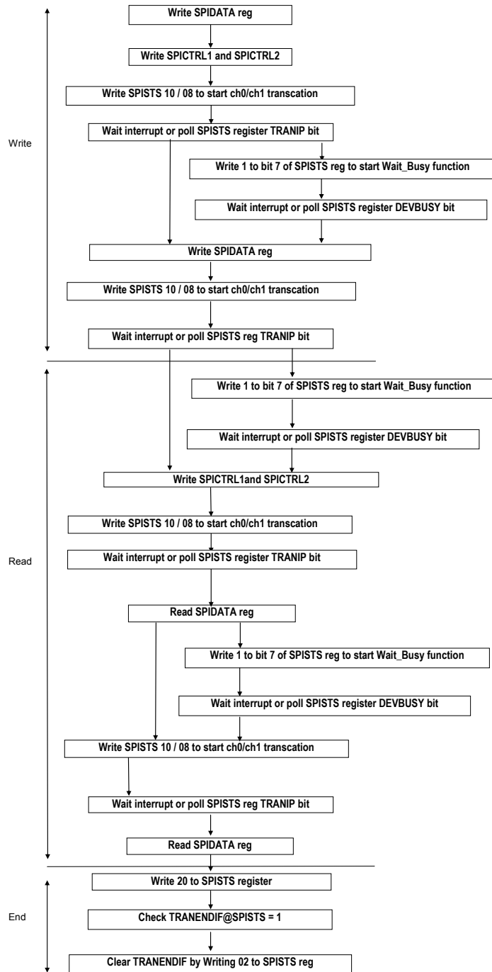
Figure 7-46. Program Flow Chart for SSPI Non-blocking
