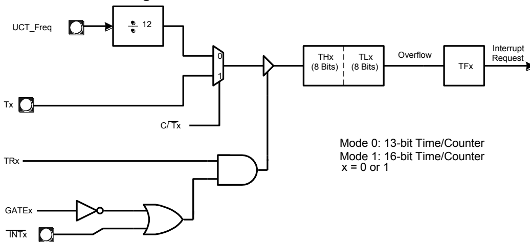
Figure 7-3. Timer 0/1 in Mode 0 and Mode 1
