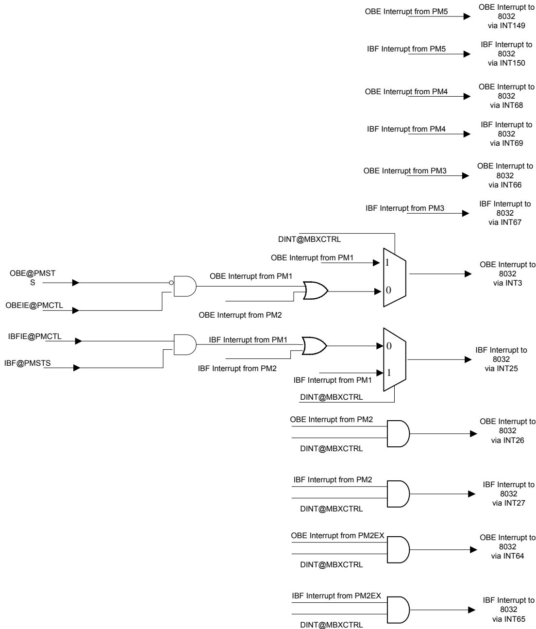
Figure 6-17. EC Interrupt Request for PMC
