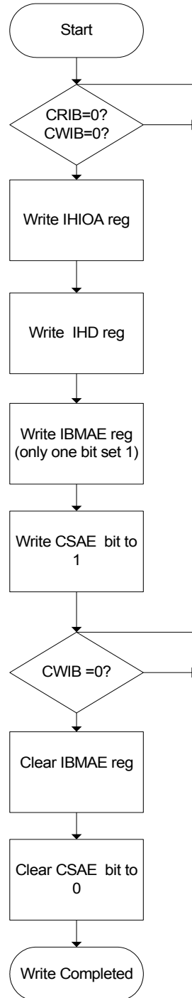
Figure 7-38. Program Flow Chart for EC2I Write
