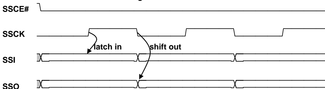
Figure 7-42. SPI Mode 0 Waveform
