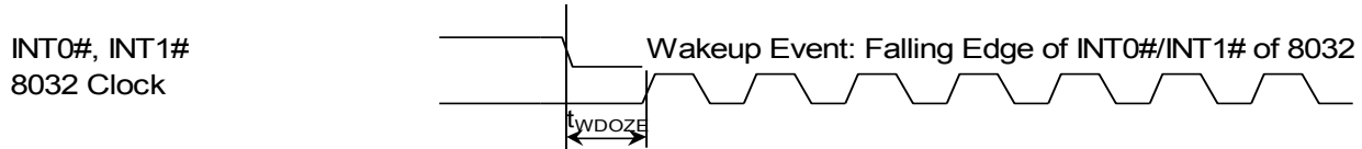
Figure 10-4. Wakeup from Doze Mode Timing
