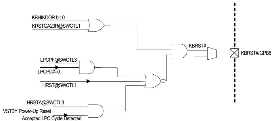
Figure 6-12. KBRST# Output Scheme
