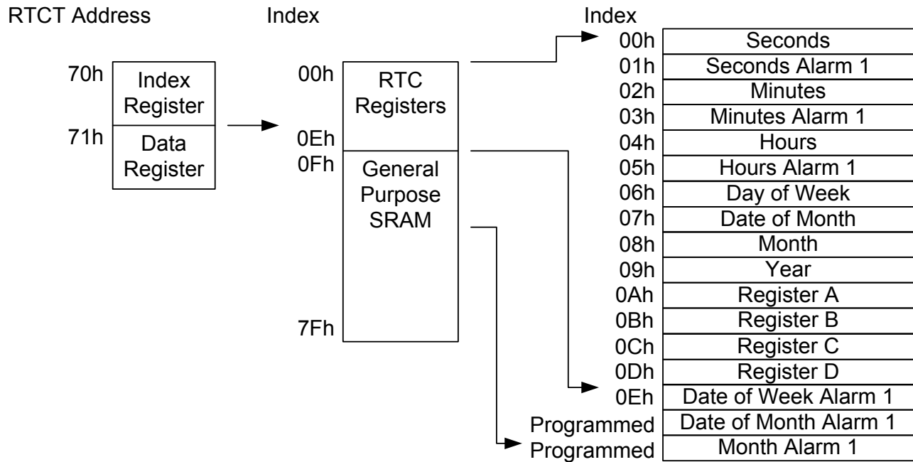
Figure 6-22. Register Map of RTCT
