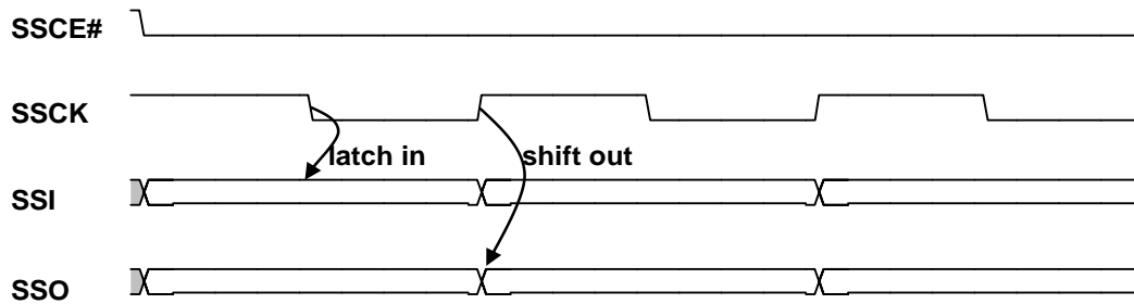
Figure 7-44. SPI Mode 2 Waveform
