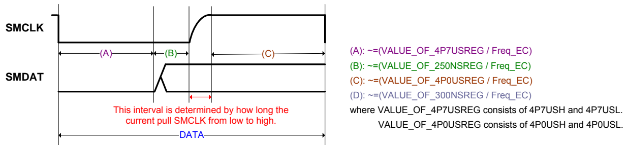
Figure 7-22. SMBus Waveform versus SMBus Timing Registers
