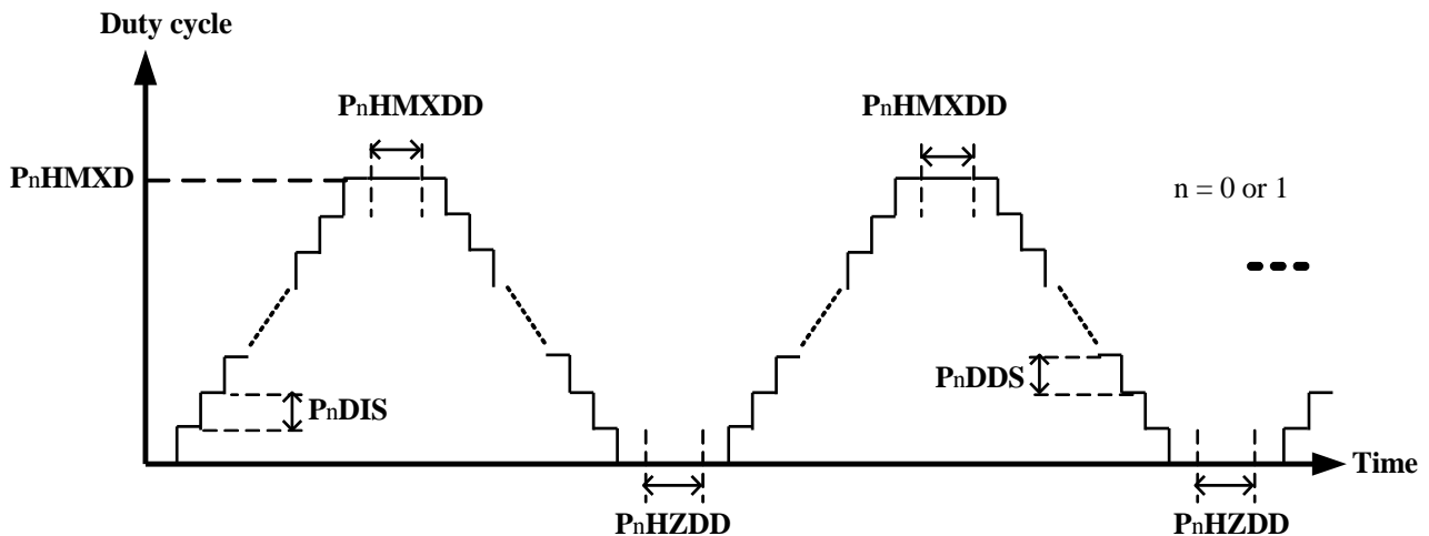
Figure 7-30. PWM LED Dimming Mode Waveform
