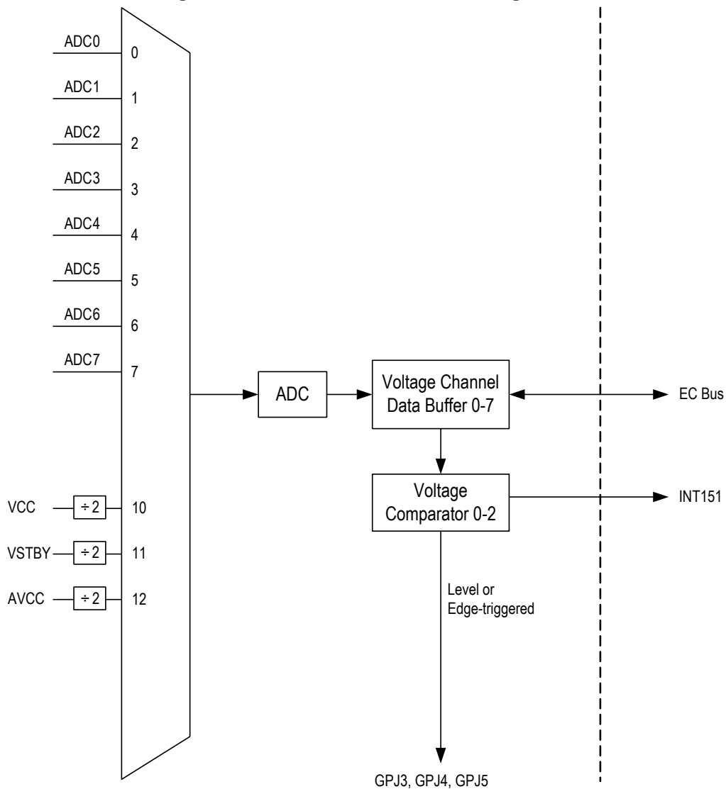
Figure 7-25. ADC Channels Control Diagram
