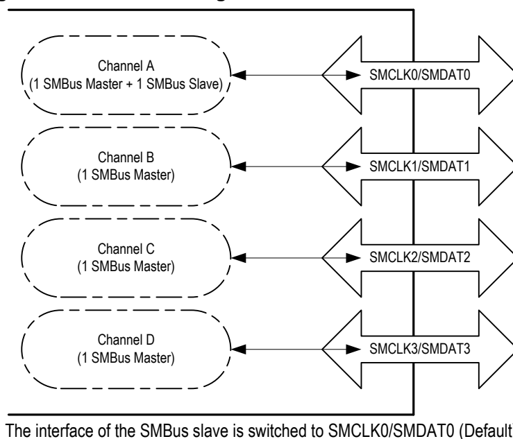
Figure 7-21. Schematic Diagram of SMBus Slave Interface Select
