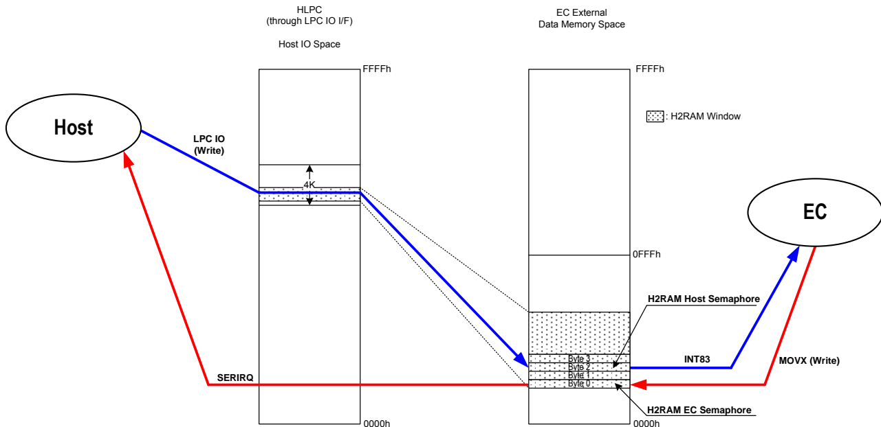
Figure 6-9. H2RAM EC/Host Semaphore Interrupt through LPC IO Cycles
