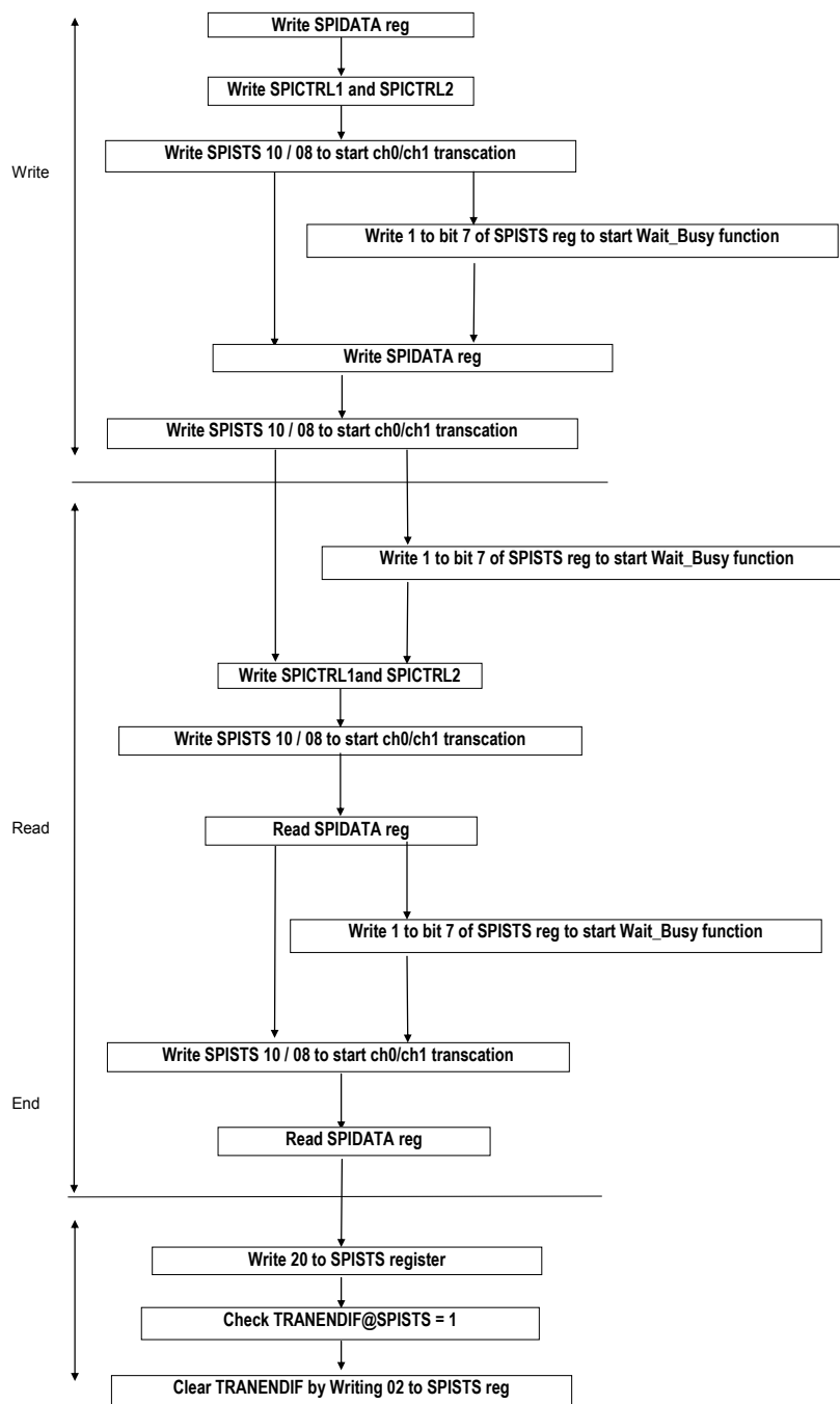
Figure 7-47. Program Flow Chart for SSPI Blocking
