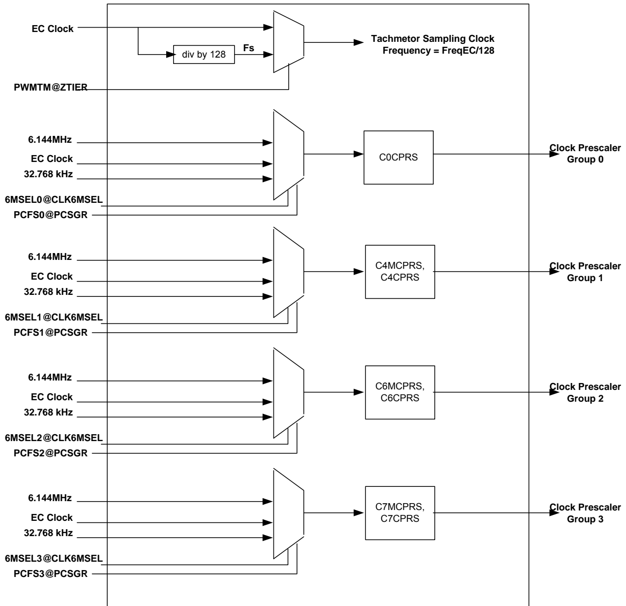
Figure 7-28. PWM Clock Tree
