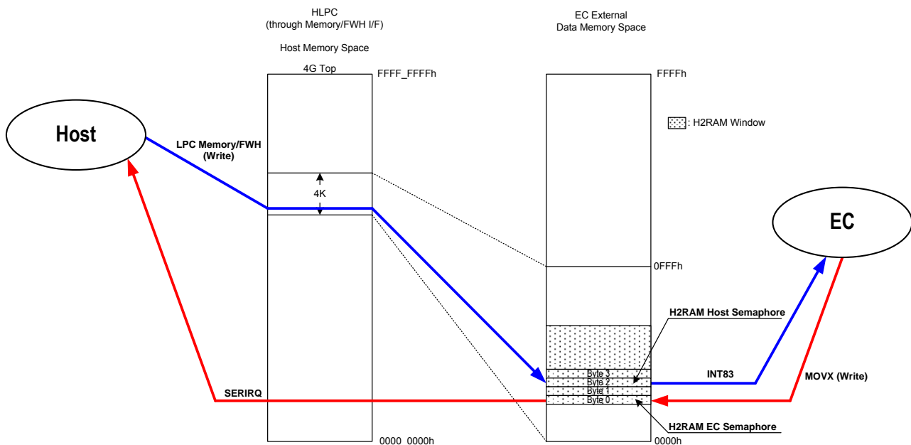
Figure 6-8. H2RAM EC/Host Semaphore Interrupt through LPC Memory/FWH Cycles
