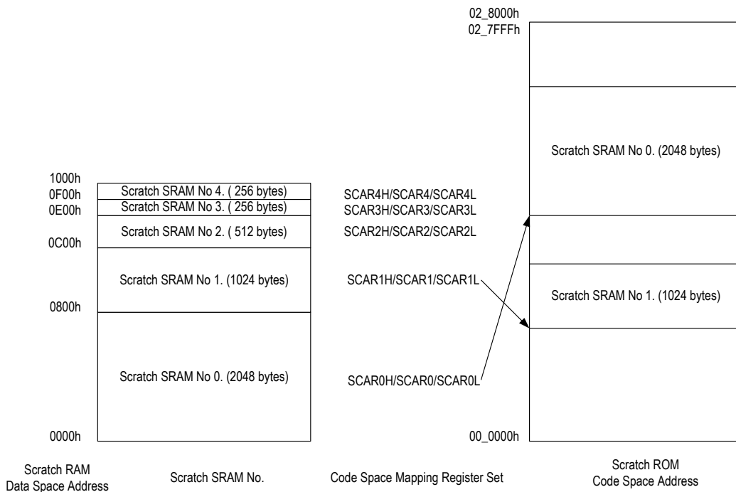
Figure 6-4. Scratch SRAM in Data Space
