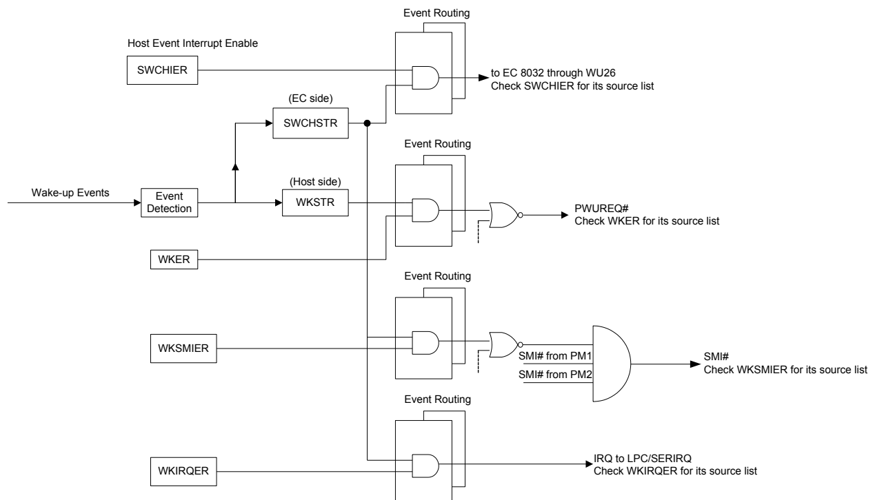
Figure 6-11. Wakeup Event and Gathering Scheme
