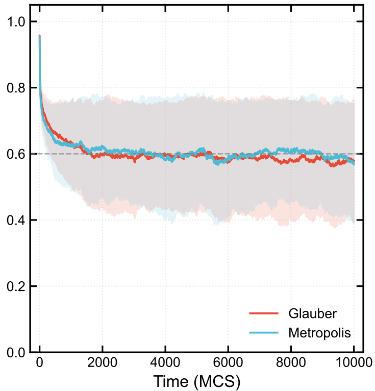
(b) T = 2.27 J/k_B , L = 64
