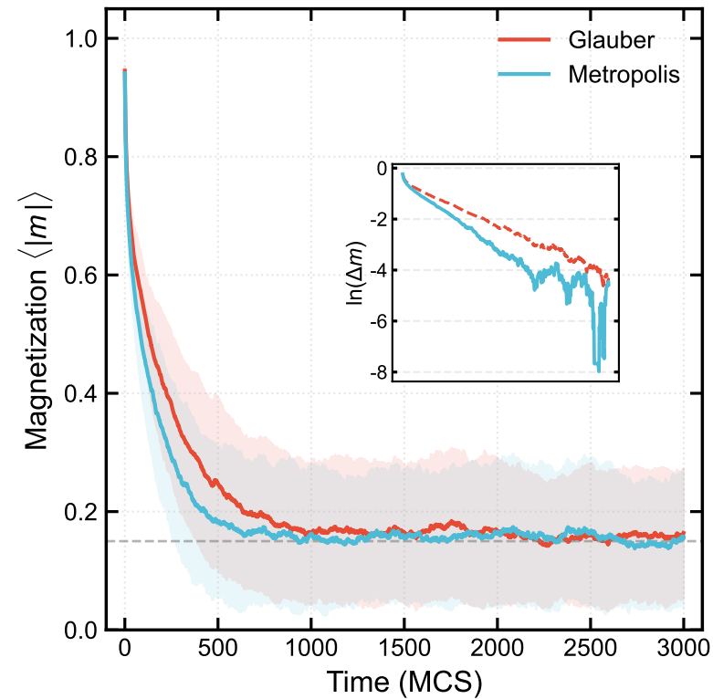
(a) T = 2.40 J/k_B , L = 64
