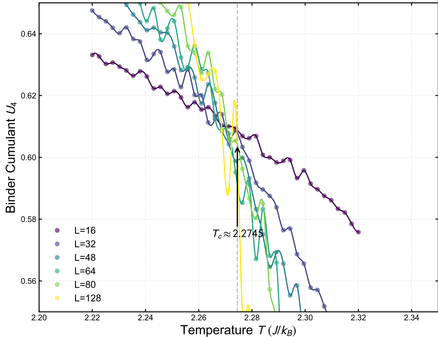
Determination of Critical Temperature T_c
