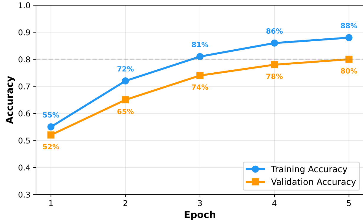
Accuracy vs Epoch
