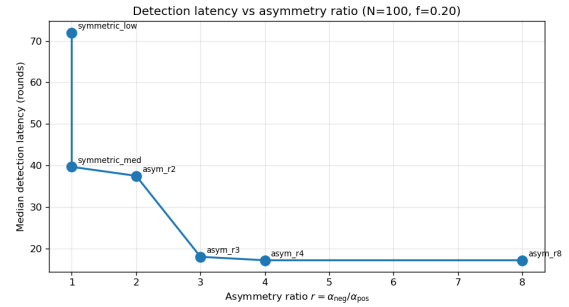
Fig. 4: Median detection latency versus asymmetry ratio r at N = 100, f = 0.20 . Six schedules are shown as labelled points spanning r \in \{1, 2, 3, 4, 8\} . The paper’s specified design point asym_r3 (at r = 3 ) sits in the steep region of the latency-vs- r curve, and the curve plateaus past r \approx 4 , confirming a saturation regime around r \geq 4 .
