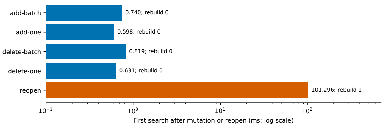
Figure 8: S1 reference RTX 4090, durable 10K×384, unfiltered B = 1 , k = 10 . Bars are first-search latency after mutation/reopen, excluding mutation/opening. Three observations per mutation type give P95; reopen is one observation. Rebuild annotations are fractions, not probabilities. Deletion checks pass. Logarithmic horizontal axis, no error bars.
