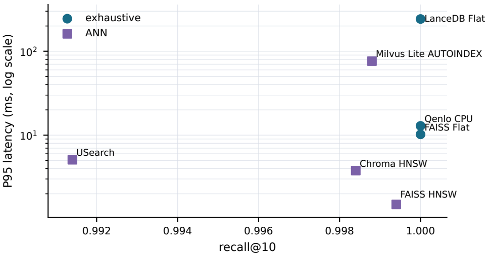
Descriptive Linux library cohort: same data and host, 1,500 calls/system
