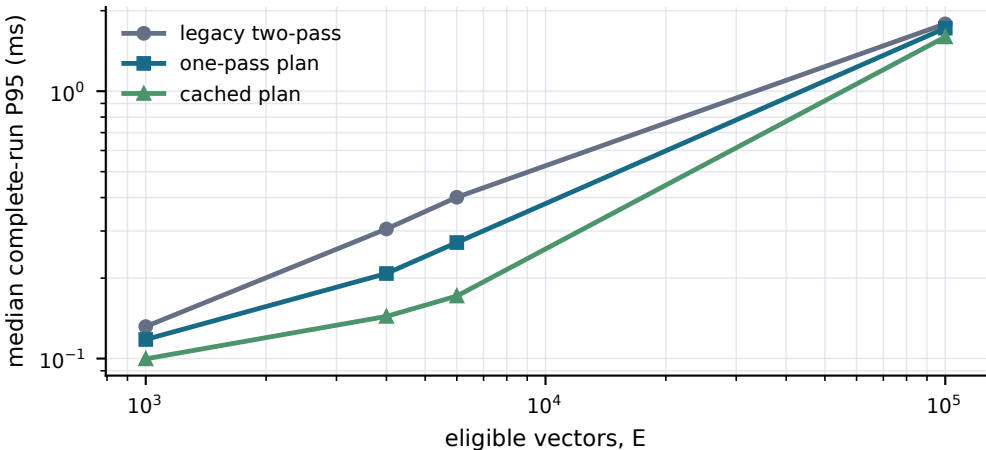
Eligibility materialization ablation, RTX 4090 / Vulkan
