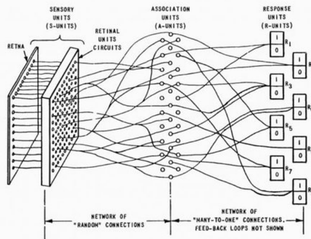
Figure 1 ORGANIZATION OF THE MARK I PFC (TRU)
