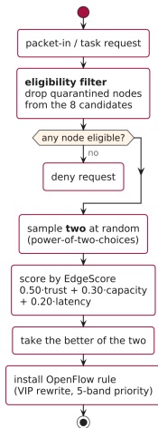
Secure load balancing — one routing decision
