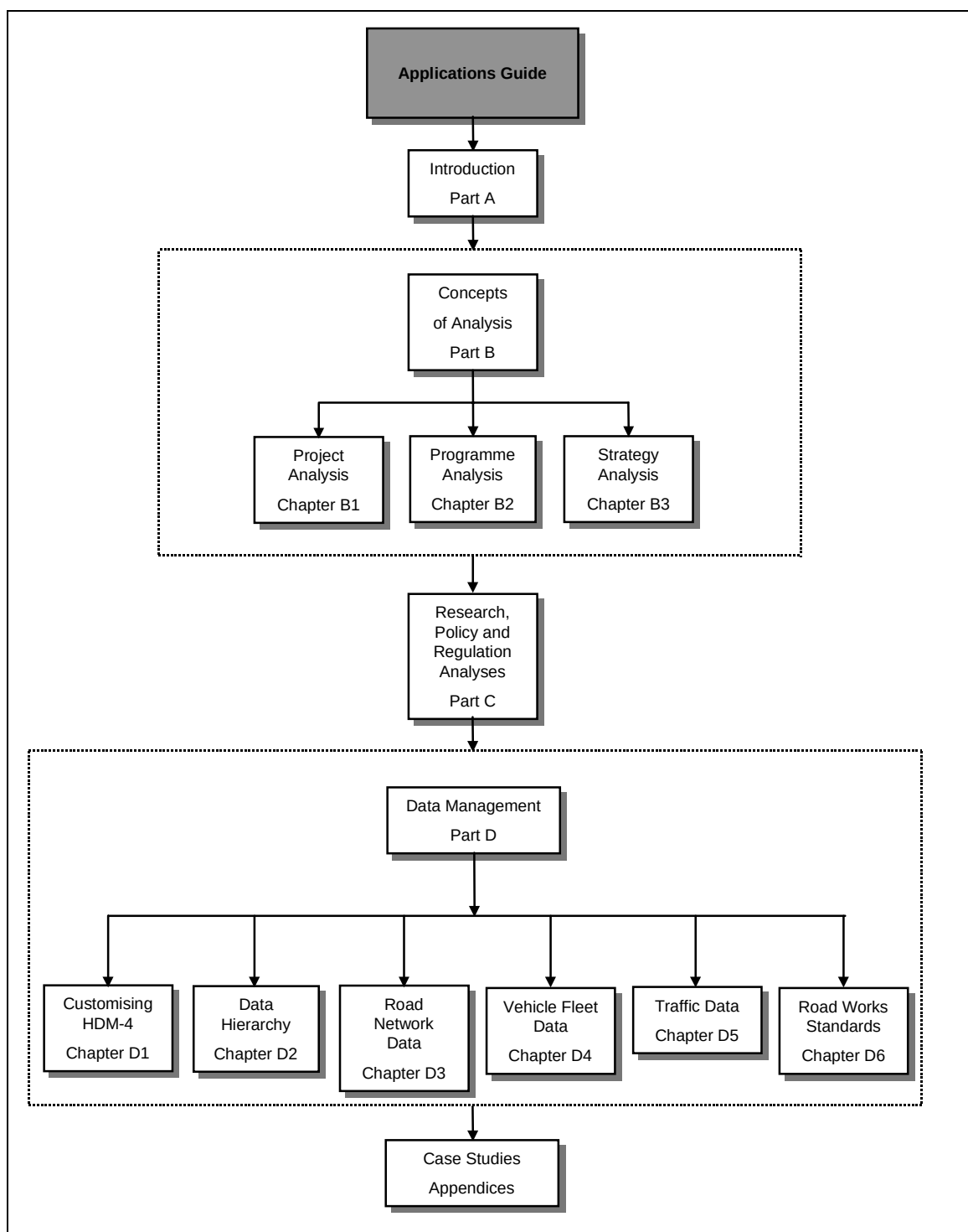
Figure 2 Schematic layout of the Applications Guide documentation
