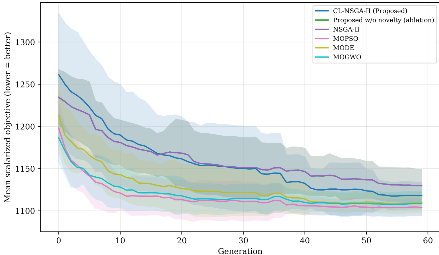
Convergence Profiles (mean \pm 1\sigma across 20 independent runs)
