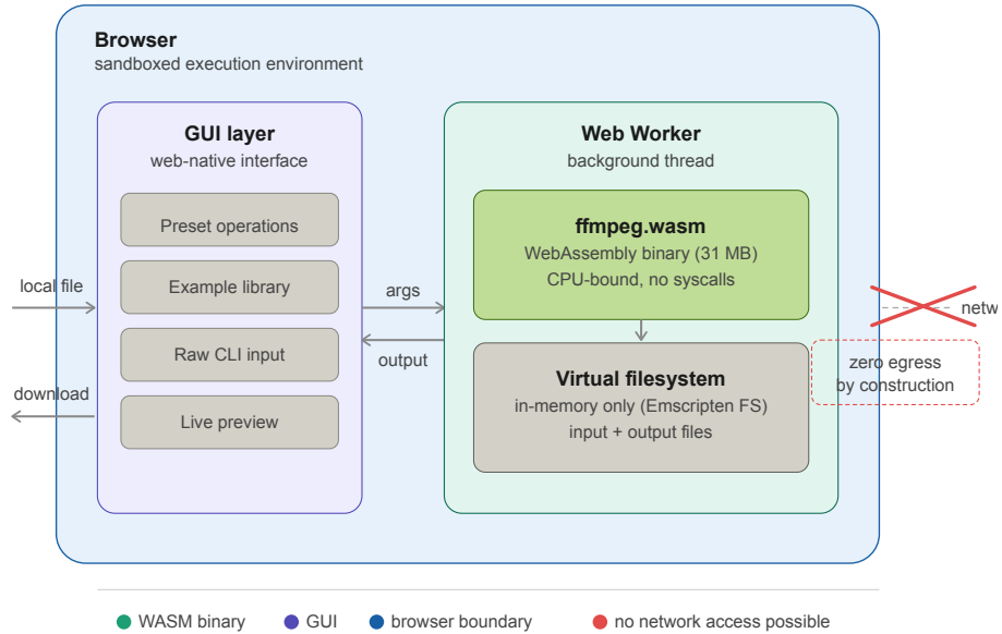
Figure 2: ffmpeg-webCLI architecture: the WASM binary executes in a Web Worker with no network access. Files are read from and written to the user's device only.
