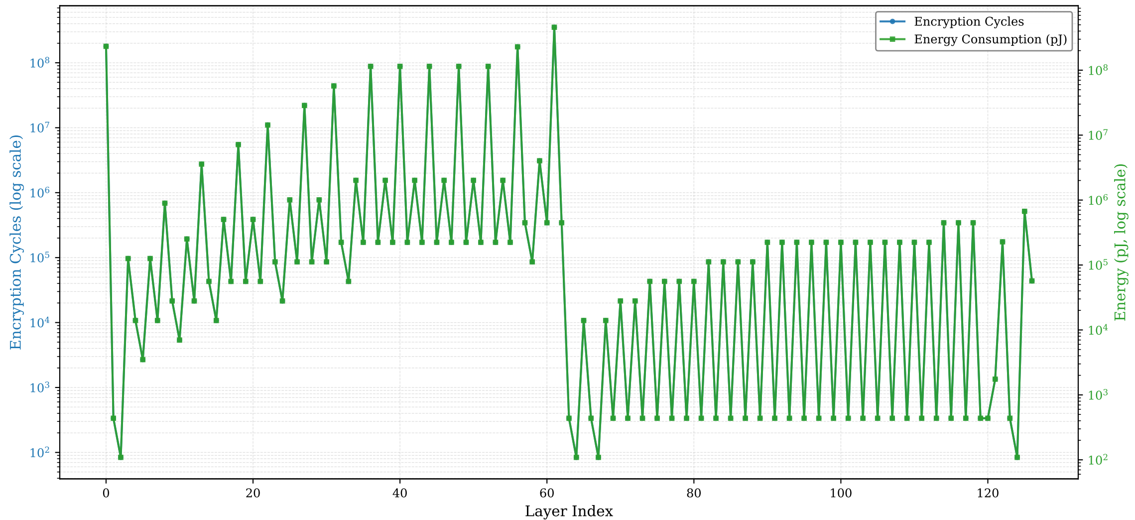
YamNet: Per-Layer Encryption Analysis (Ascon)
