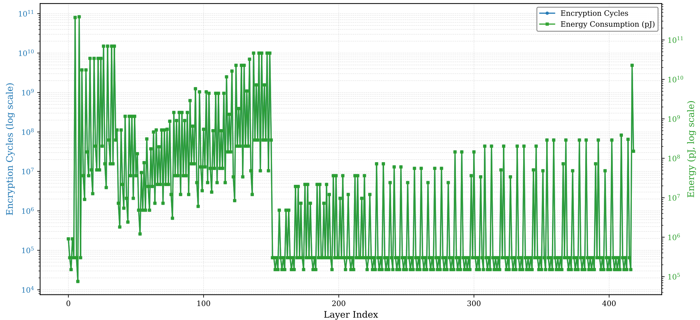
mobile_netv3: Per-Layer Encryption Analysis (Grain128)
