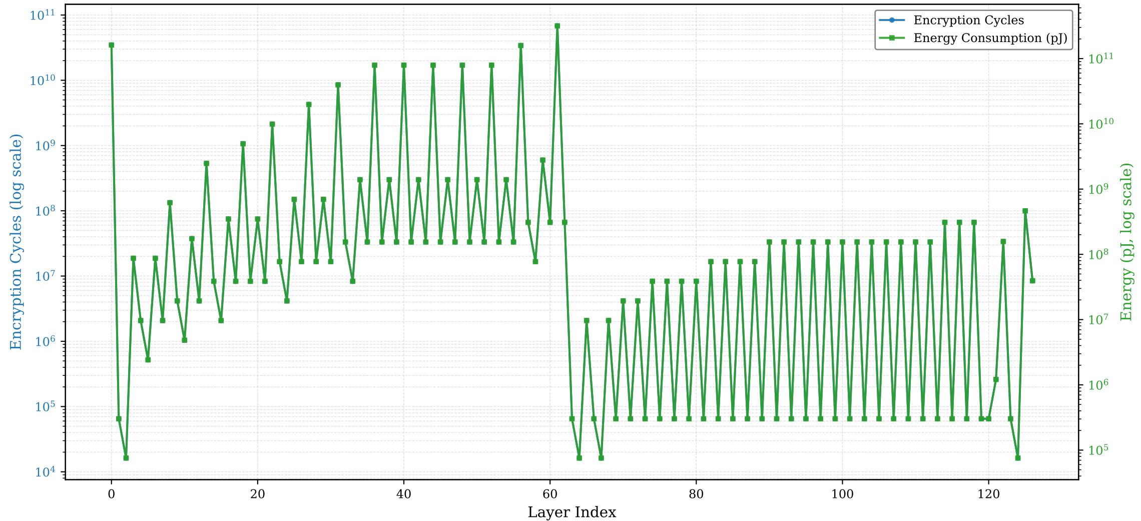
YamNet: Per-Layer Encryption Analysis (Grain128)
