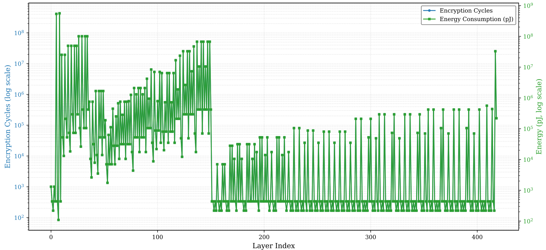
mobile_netv3: Per-Layer Encryption Analysis (Ascon)
