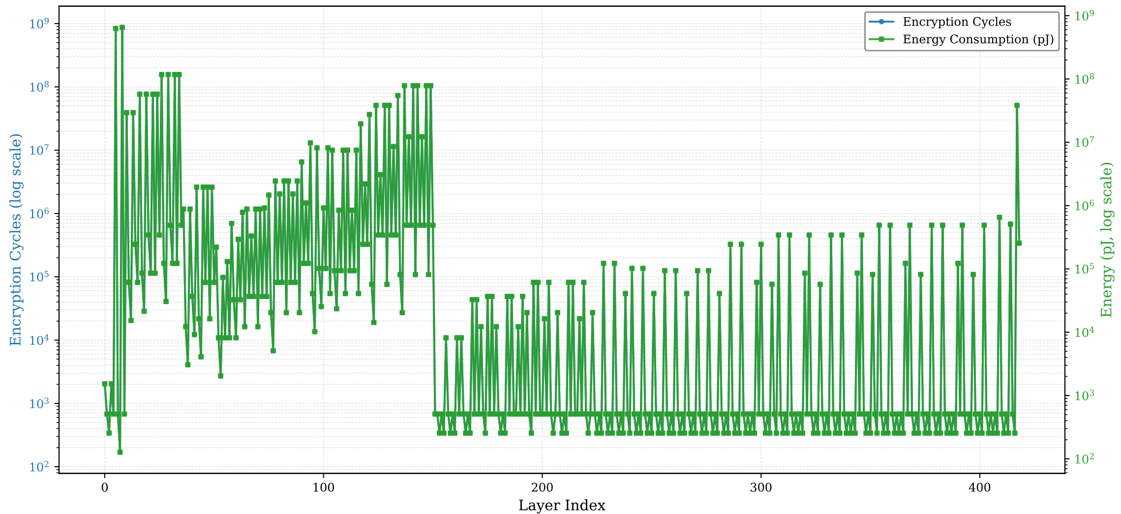
mobile_netv3: Per-Layer Encryption Analysis (Chacha20 Poly1305)
