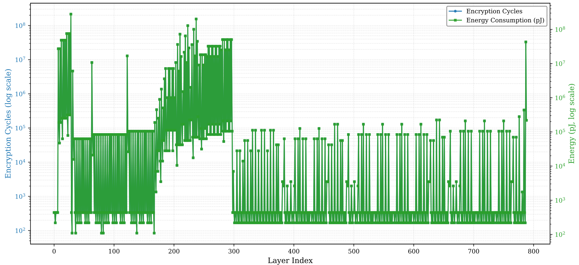
mobile_vit: Per-Layer Encryption Analysis (Ascon)
