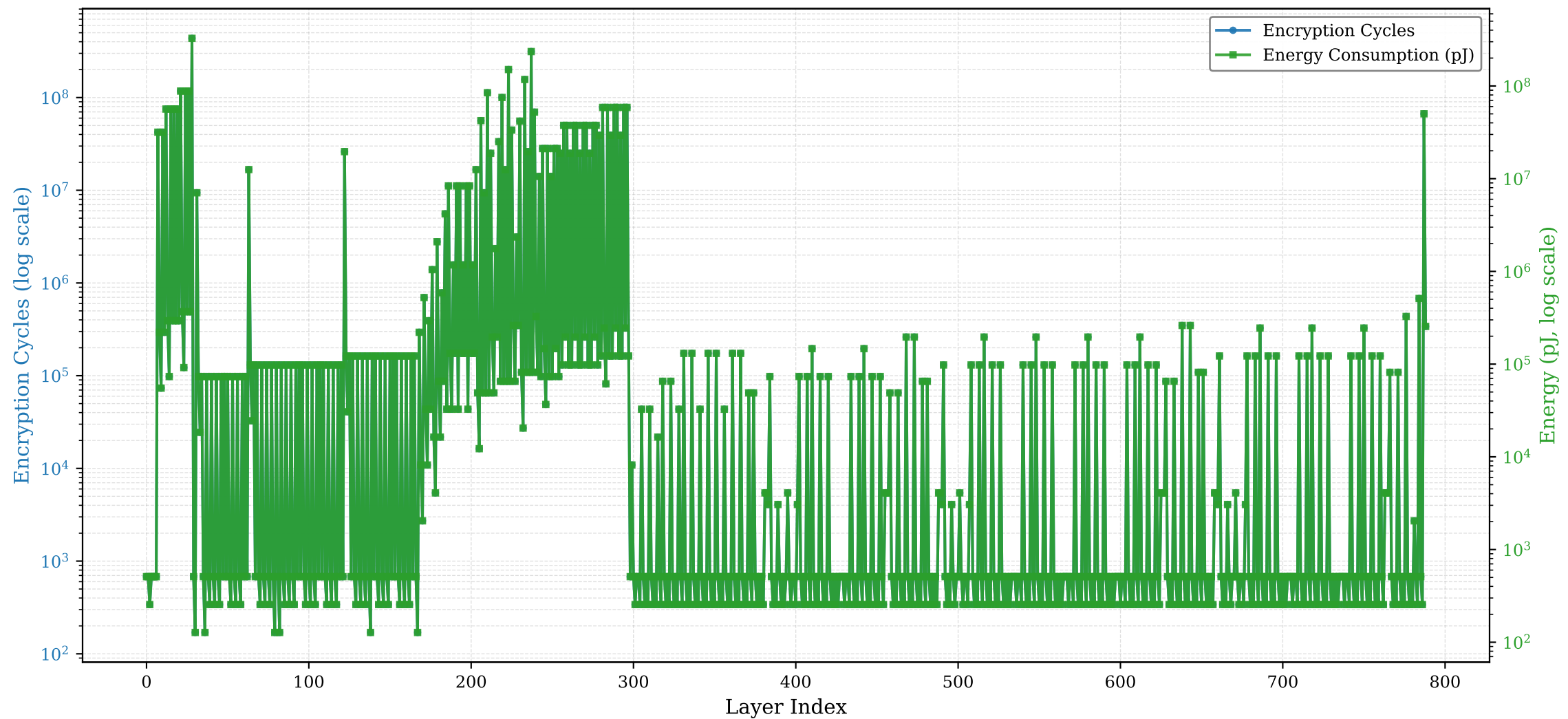
mobile_vit: Per-Layer Encryption Analysis (Chacha20 Poly1305)
