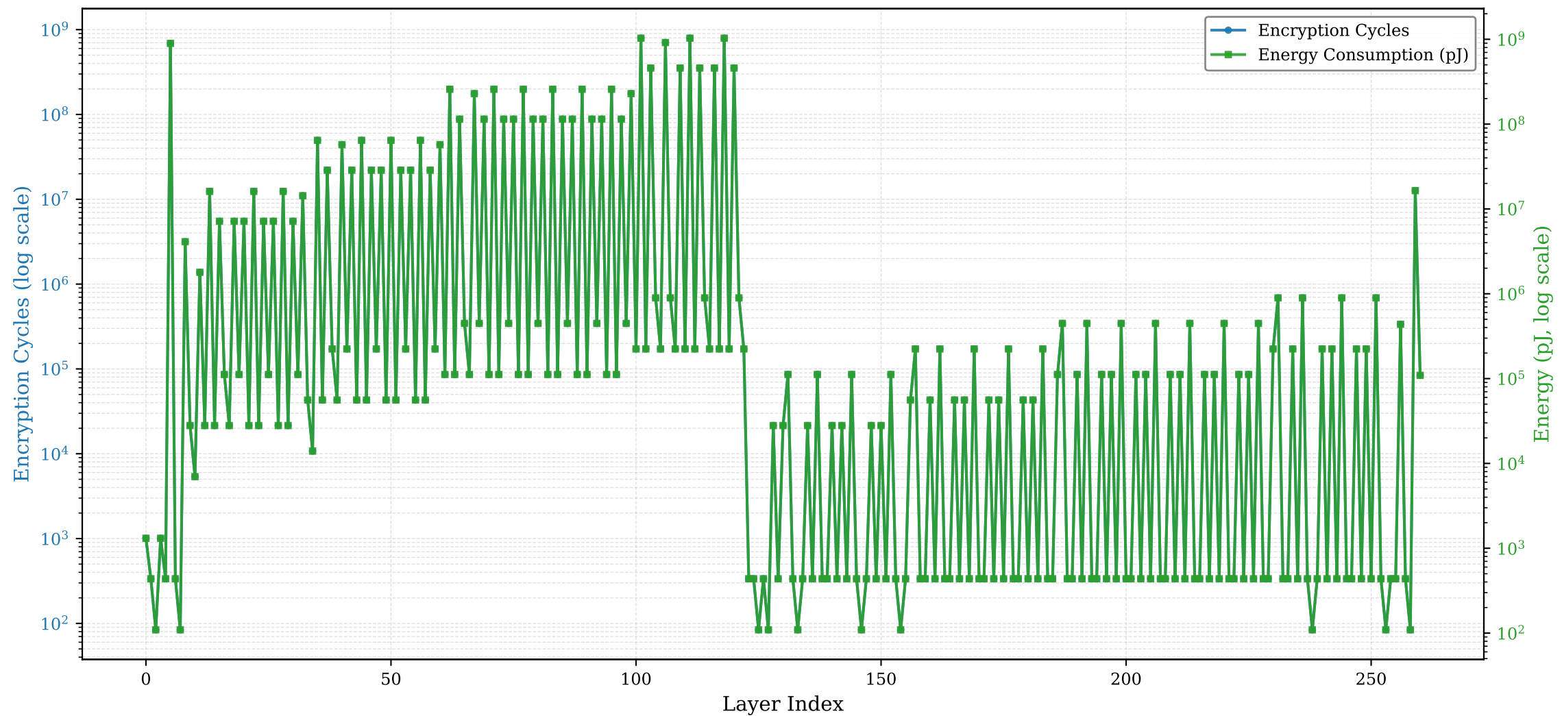
resnet50: Per-Layer Encryption Analysis (Ascon)
