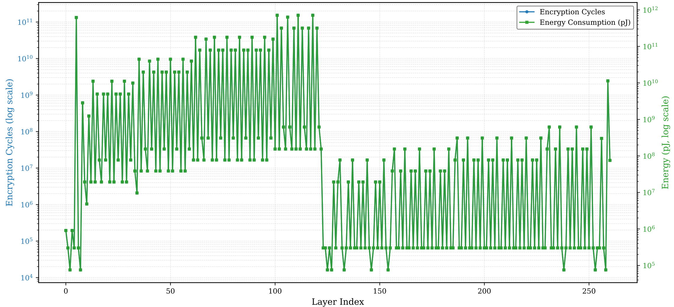
resnet50: Per-Layer Encryption Analysis (Grain128)
