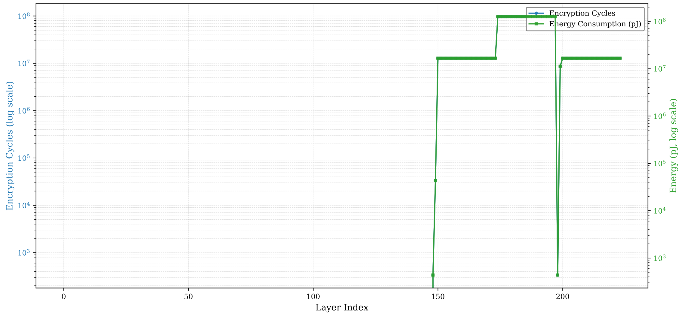
whisper_decoder: Per-Layer Encryption Analysis (Ascon)
