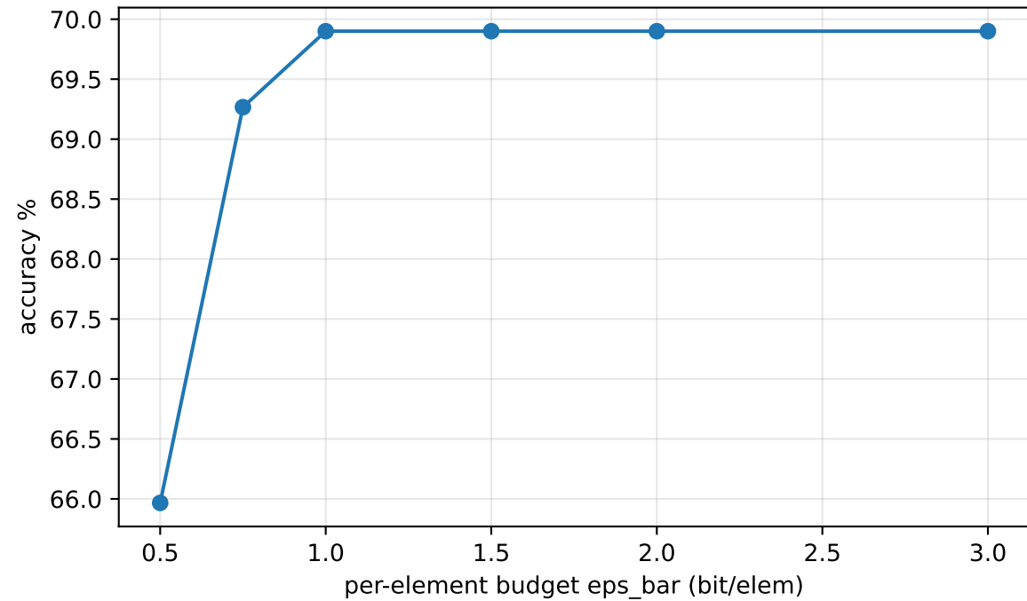
Privacy-utility frontier
