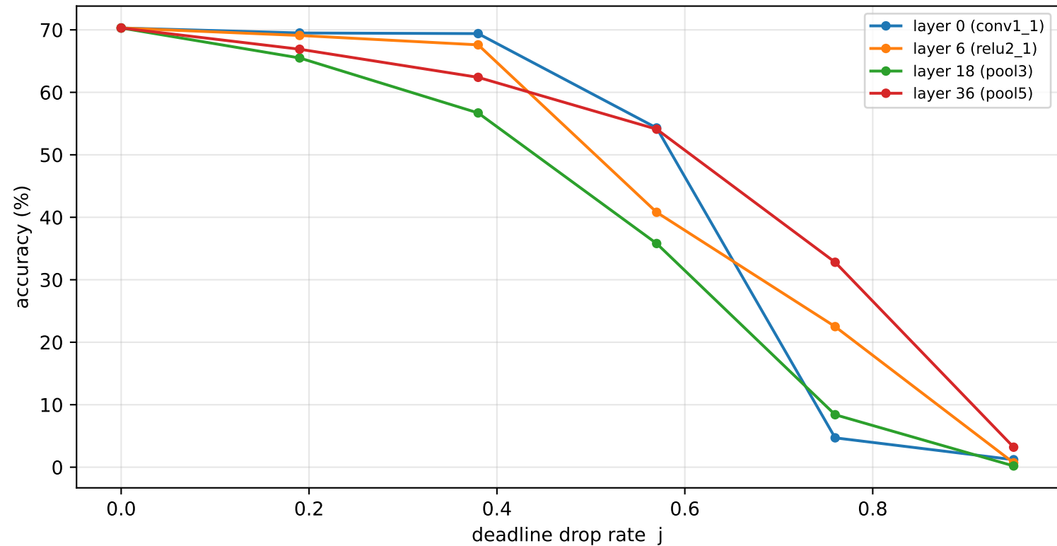
Accuracy vs Drop Rate (deadline truncation), per split layer
