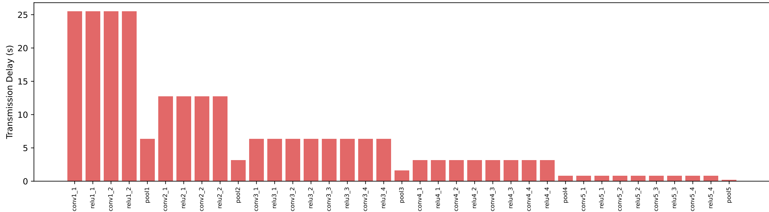
Fig. 2 — Transmission delay per split layer (BSE = PA-BSE, privacy-invariant)
