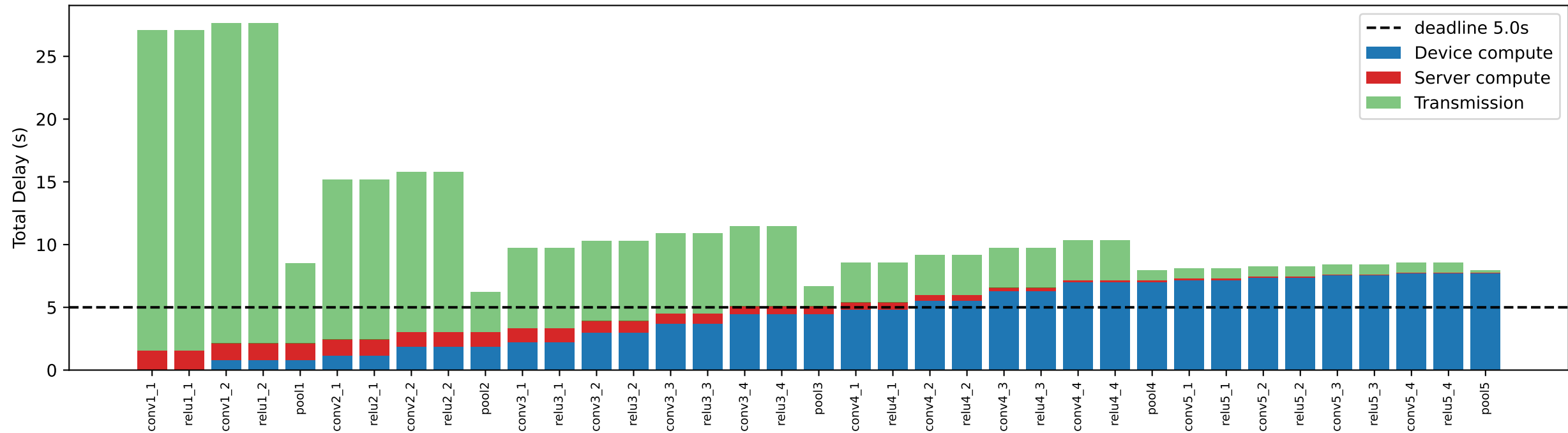
Fig. 3 — End-to-end delay breakdown (BSE = PA-BSE)
