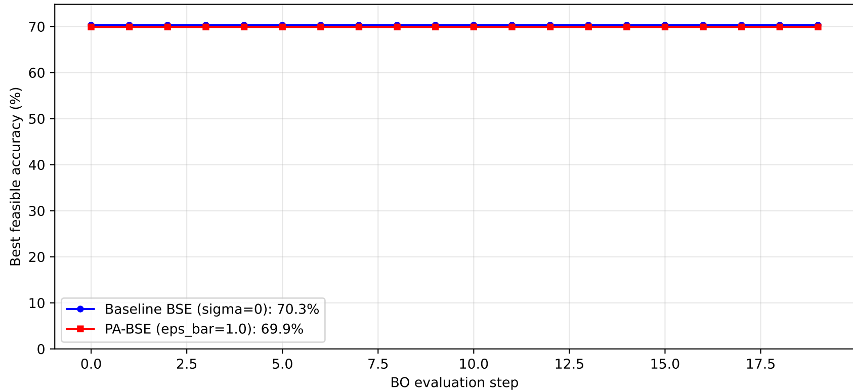
Fig. 6 — Accuracy vs evaluation step (BSE vs PA-BSE)
