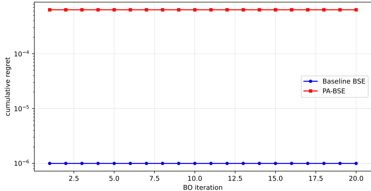
Fig. 8 — Cumulative regret (BSE vs PA-BSE)
