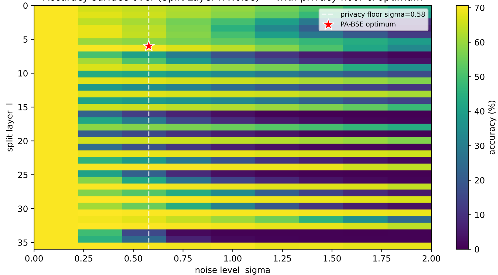
Accuracy surface over (Split Layer x Noise) — with privacy floor & optimum
