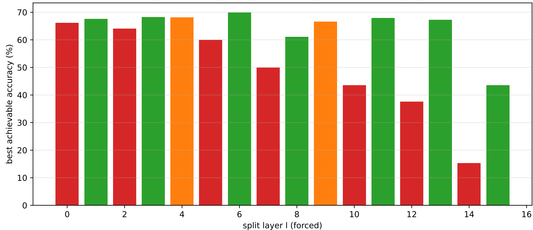
Item 2 — accuracy when each split layer is forced (green=relu, orange=pool, red=conv)
