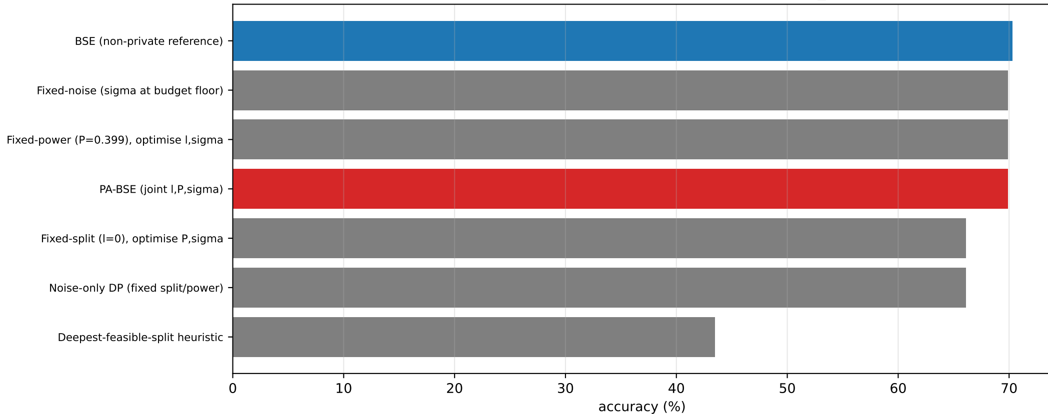
Item 3 — PA-BSE vs privacy-preserving baselines (eps_bar=1.0)
