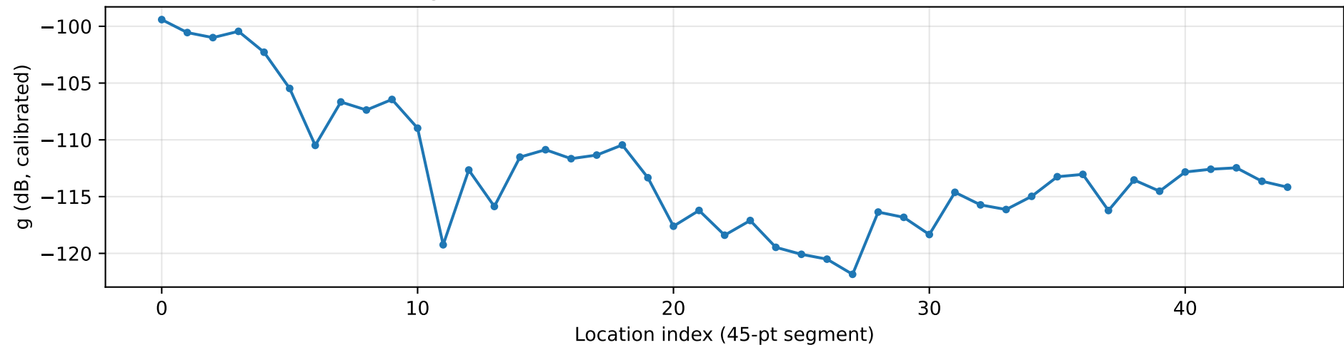
Channel gains (calibrated) — mMMobile outdoor 30m (loc=1, beam=1)
