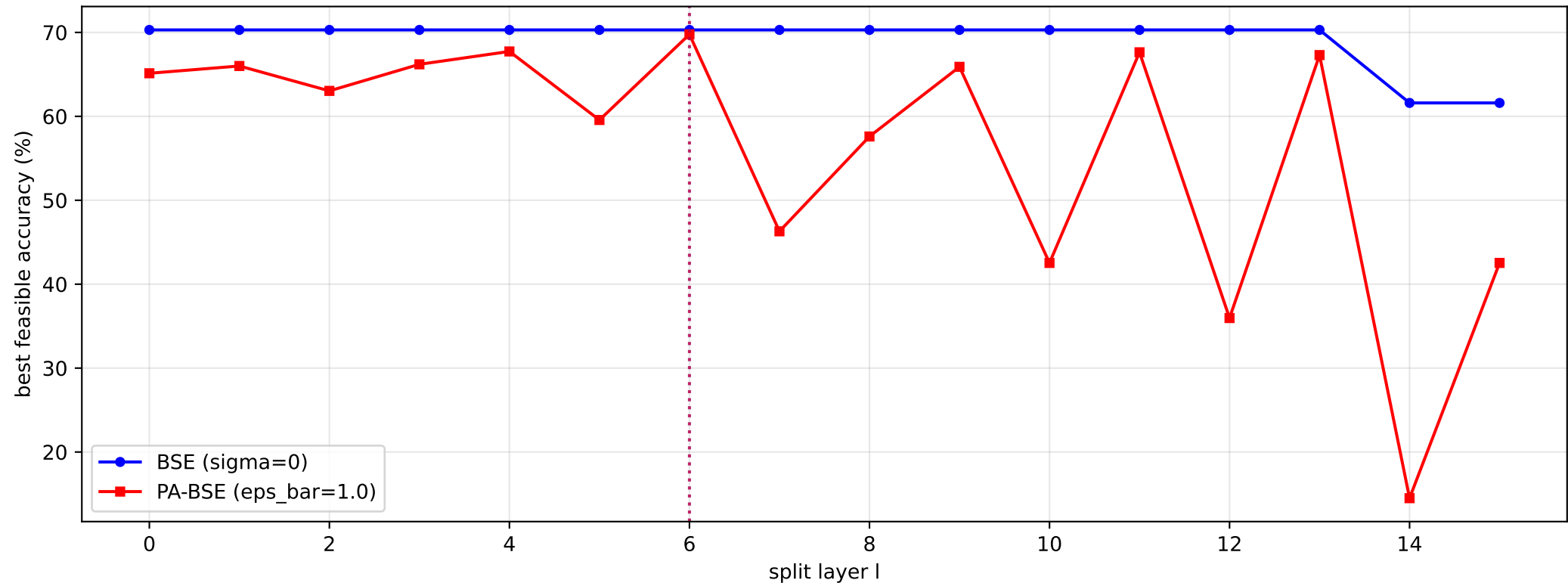
NEW — Accuracy vs Split Layer: PA-BSE vs BSE
