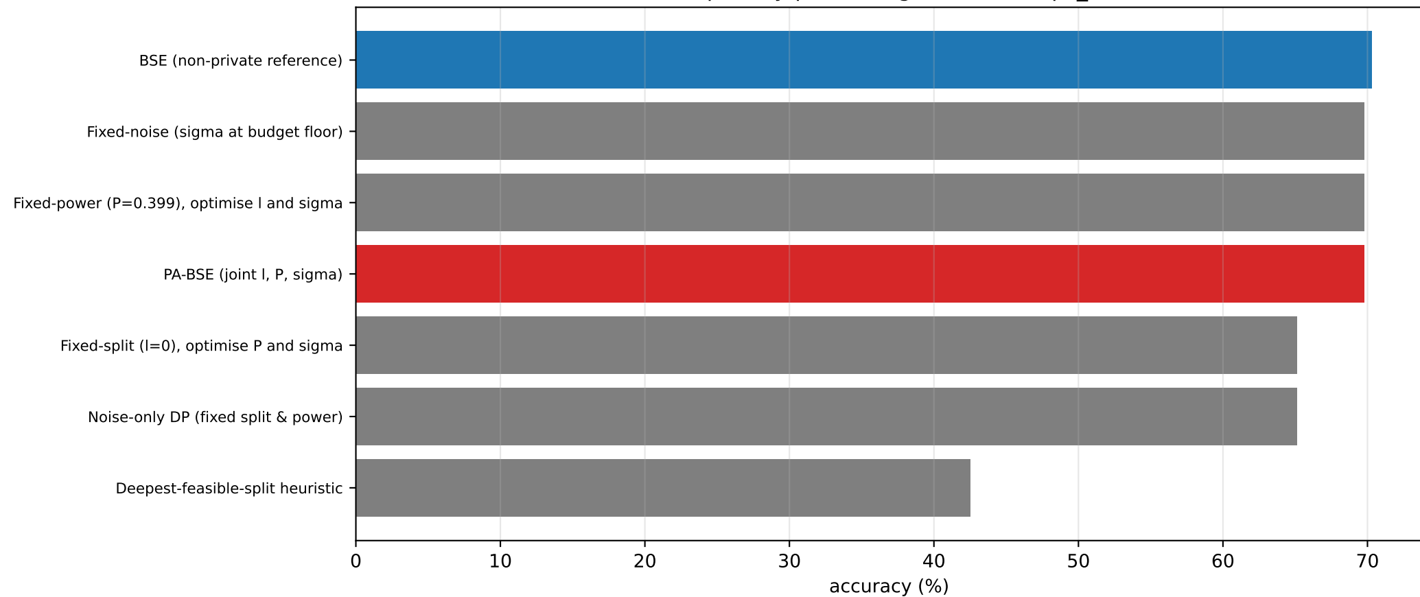
PA-BSE vs privacy-preserving baselines (eps_bar=1.0)
