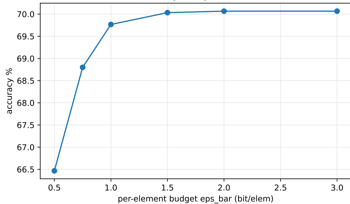
Privacy-utility frontier
