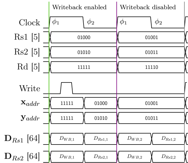
Figure 3: Thorn-2 register file timing diagram.
