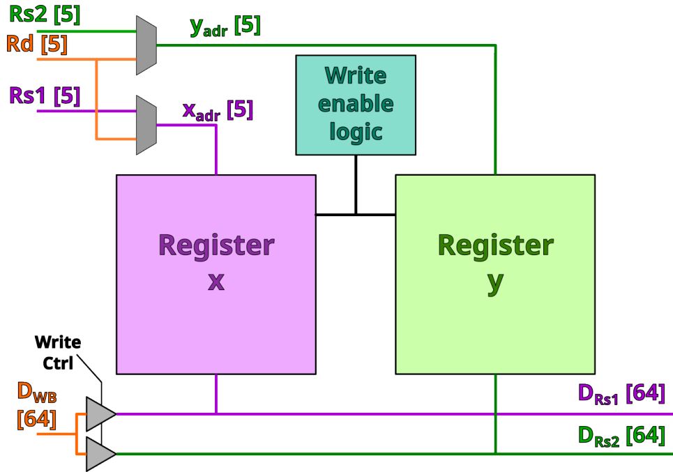
Figure 2: The Thorn-2 register file.
