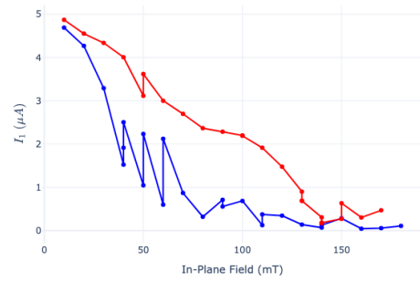
1st Harmonic Amplitude vs In-Plane Field
