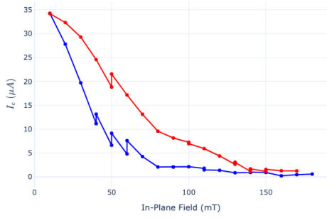
Critical Current vs In-Plane Field
