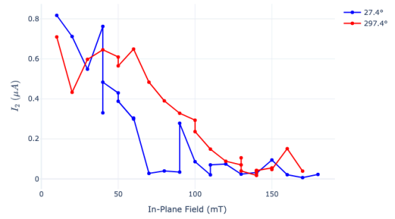
2nd Harmonic Amplitude vs In-Plane Field
