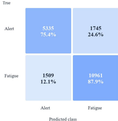
Classification confusion matrix
