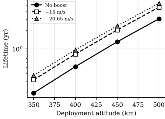
Fig. 7. Orbital lifetime vs deployment altitude (BC = 61 kg/m 2 , mean activity).
