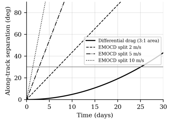
Fig. 9. Constellation seeding: EMOCD velocity splits versus differential drag under identical assumptions.
