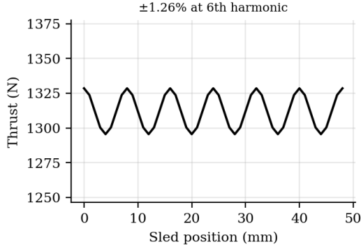
Fig. 4. Winding-resolved thrust over one wavelength of sled travel.
