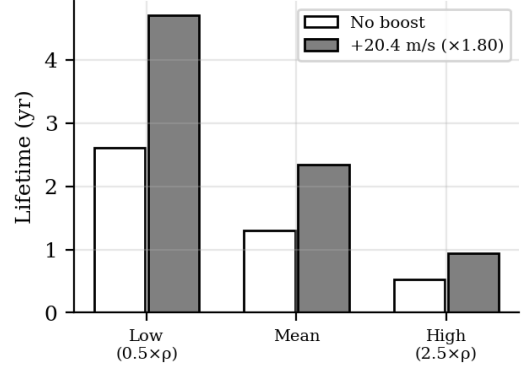
Fig. 8. Solar-activity sweep: absolute lifetimes vary fivefold; the \times 1.8 multiplier does not.
