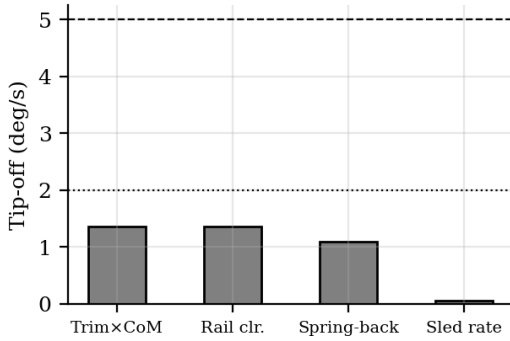
Fig. 11. Tip-off error budget against deployer requirement classes.
