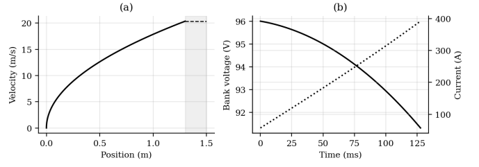
Fig. 5. Shot profile at the rated point: (a) velocity with coast-trim zone; (b) bank voltage and current.
