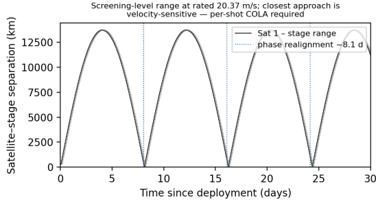
Fig. 10. Satellite-stage range over 30 days, staggered firing at the rated velocity.
