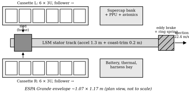
Fig. 2. Plan-view layout within an ESPA-Grande-class envelope (not to scale).
