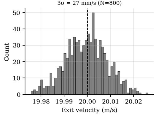
Fig. 6. Closed-loop exit-velocity dispersion, 800 Monte Carlo runs.
